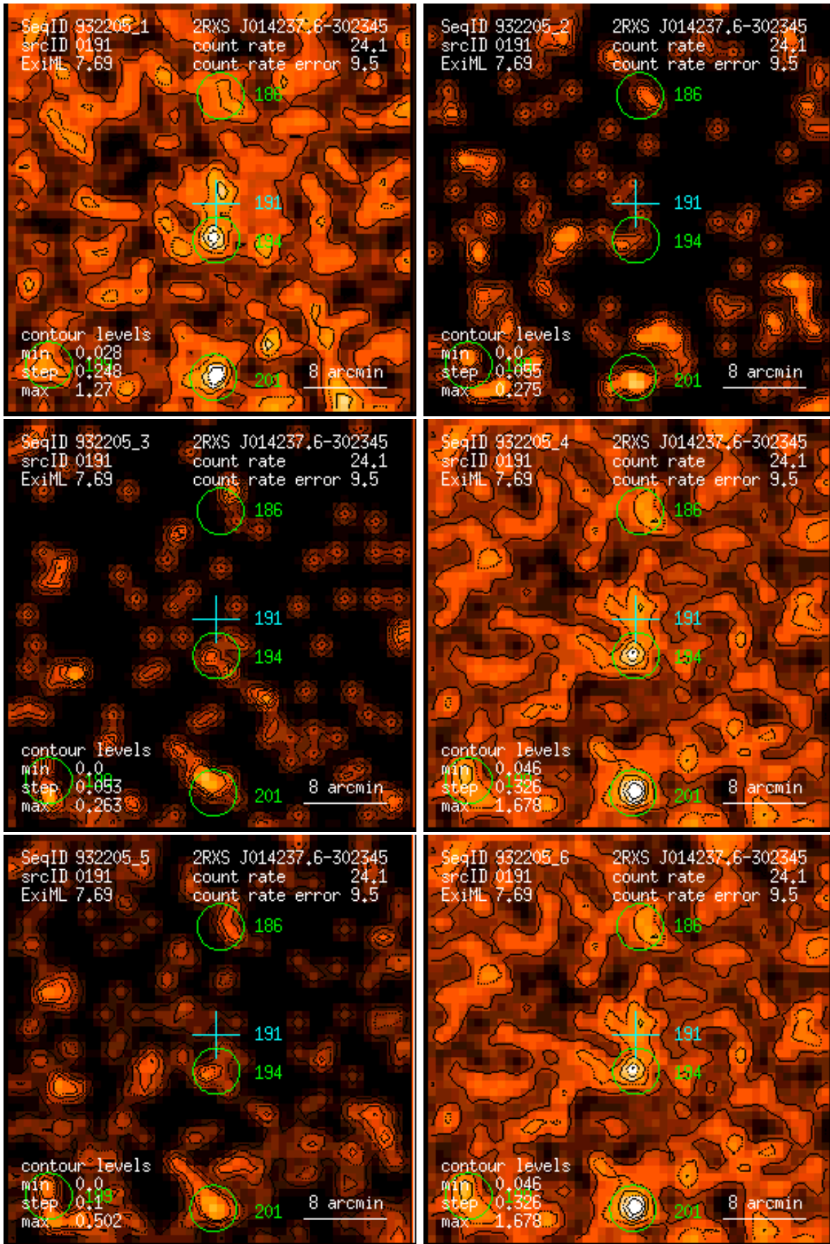
Figure 191: RASS 932205: detection 0191: band rate images, Gaussian filter: (1) PSPC channels 11 – 41, (2) 52 – 90, (3) 91 – 201, (4) 11 – 235, (5) 52 – 201, (6) 11 – 201. Broad band rates in counts/ks. Band rate contour levels in counts/ks/arcmin 2 .
