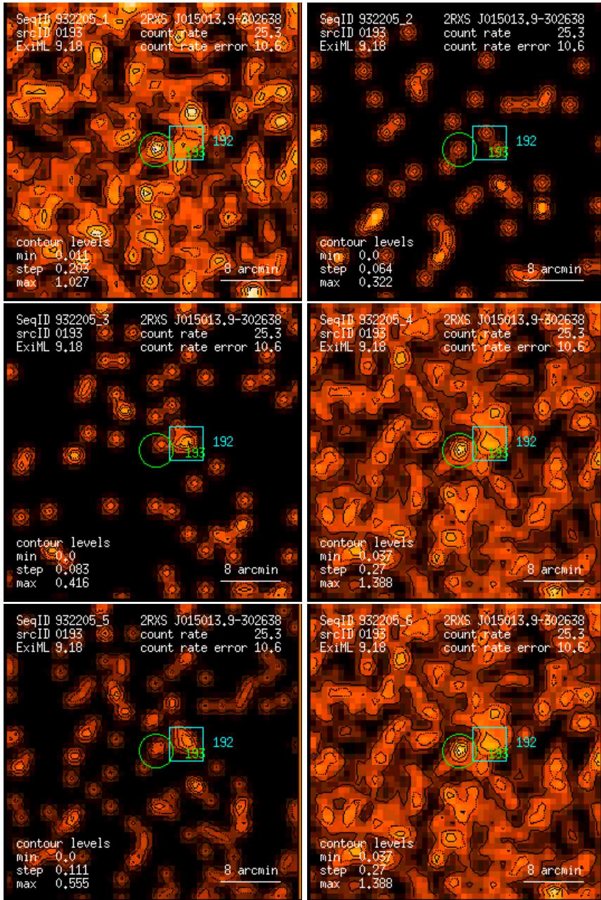
Figure 193: RASS 932205: detection 0193: band rate images, Gaussian filter: (1) PSPC channels 11 – 41, (2) 52 – 90, (3) 91 – 201, (4) 11 – 235, (5) 52 – 201, (6) 11 – 201. Broad band rates in counts/ks. Band rate contour levels in counts/ks/arcmin 2 .
