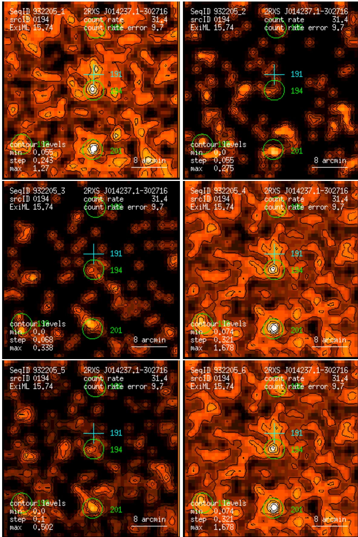
Figure 194: RASS 932205: detection 0194: band rate images, Gaussian filter: (1) PSPC channels 11 – 41, (2) 52 – 90, (3) 91 – 201, (4) 11 – 235, (5) 52 – 201, (6) 11 – 201. Broad band rates in counts/ks. Band rate contour levels in counts/ks/arcmin 2 .
