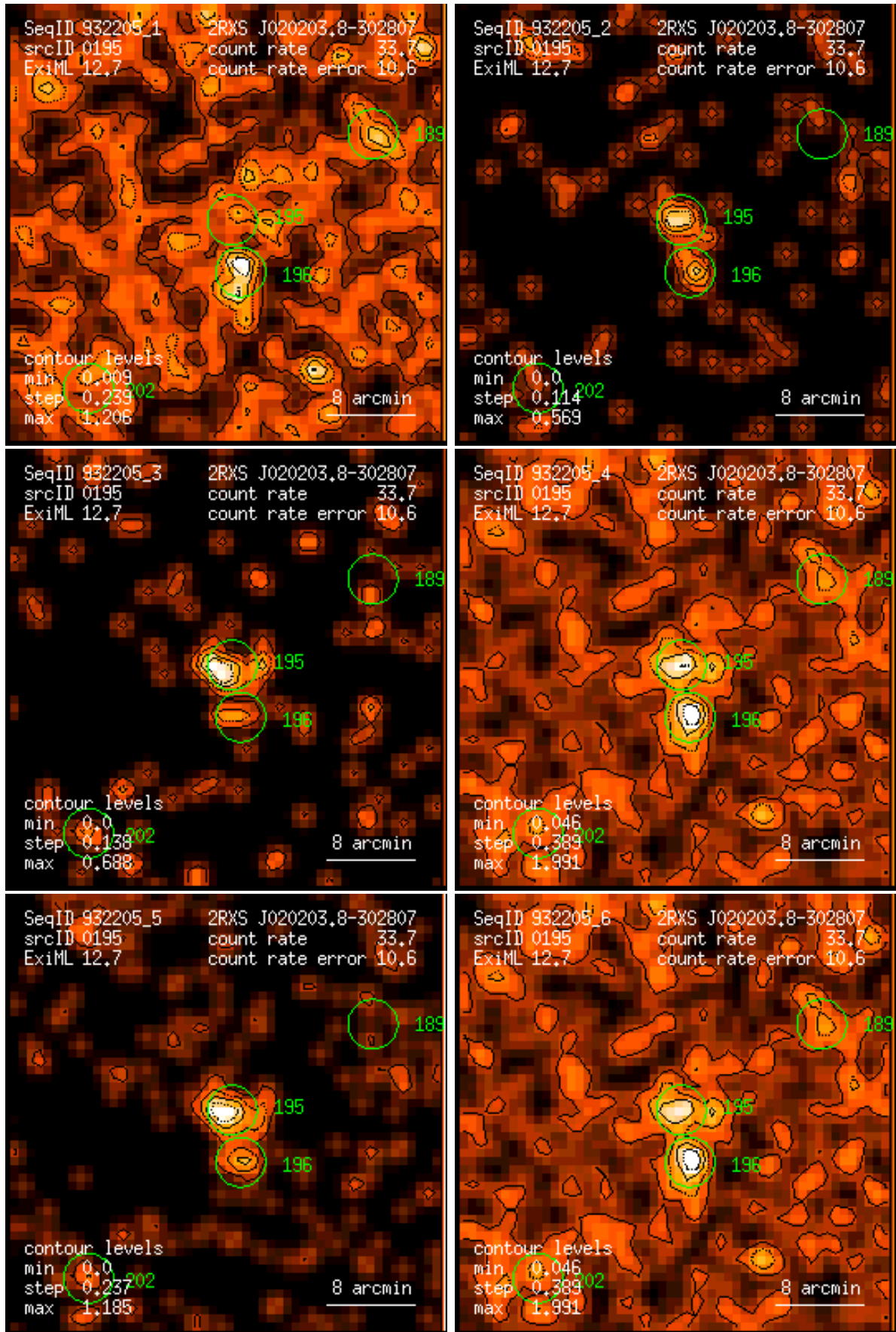
Figure 195: RASS 932205: detection 0195: band rate images, Gaussian filter: (1) PSPC channels 11 – 41, (2) 52 – 90, (3) 91 – 201, (4) 11 – 235, (5) 52 – 201, (6) 11 – 201. Broad band rates in counts/ks. Band rate contour levels in counts/ks/arcmin 2 .
