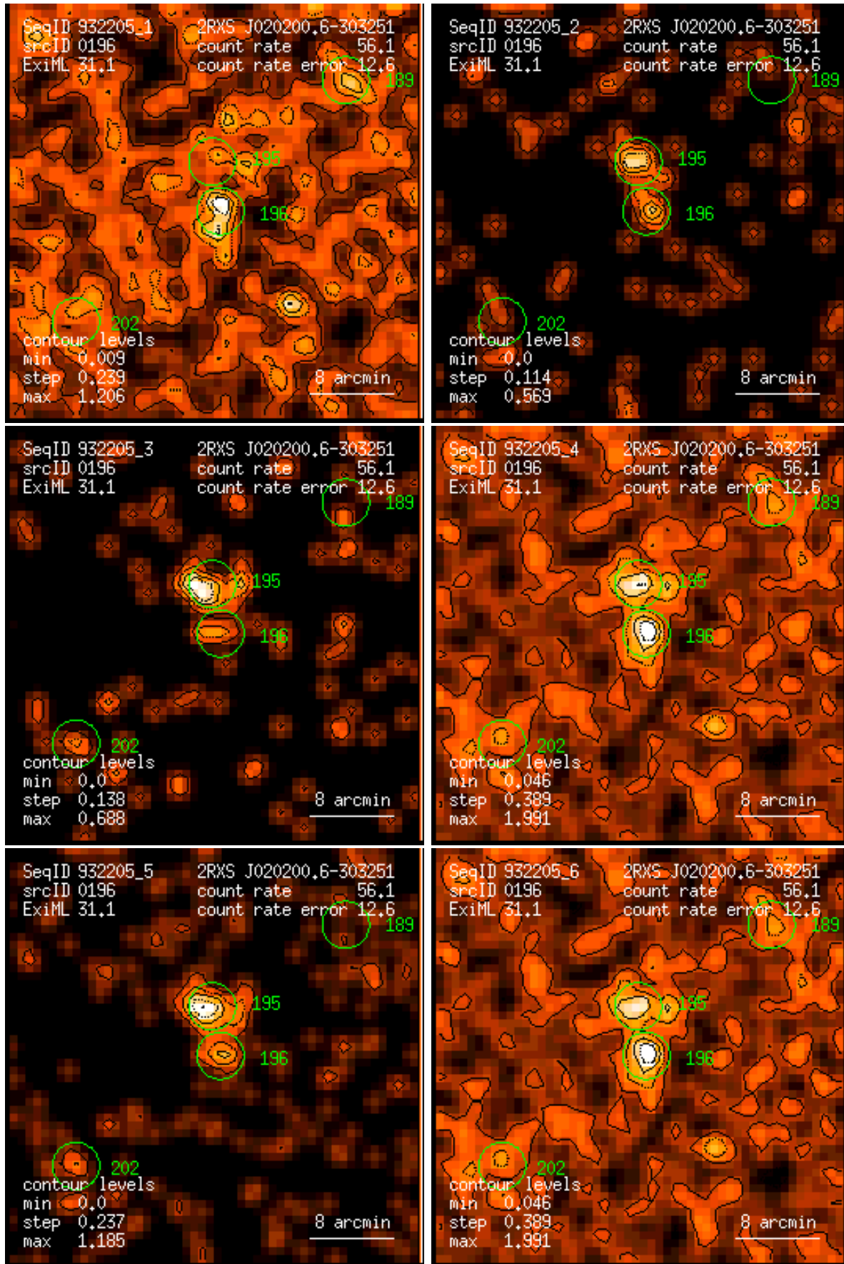
Figure 196: RASS 932205: detection 0196: band rate images, Gaussian filter: (1) PSPC channels 11 – 41, (2) 52 – 90, (3) 91 – 201, (4) 11 – 235, (5) 52 – 201, (6) 11 – 201. Broad band rates in counts/ks. Band rate contour levels in counts/ks/arcmin 2 .
