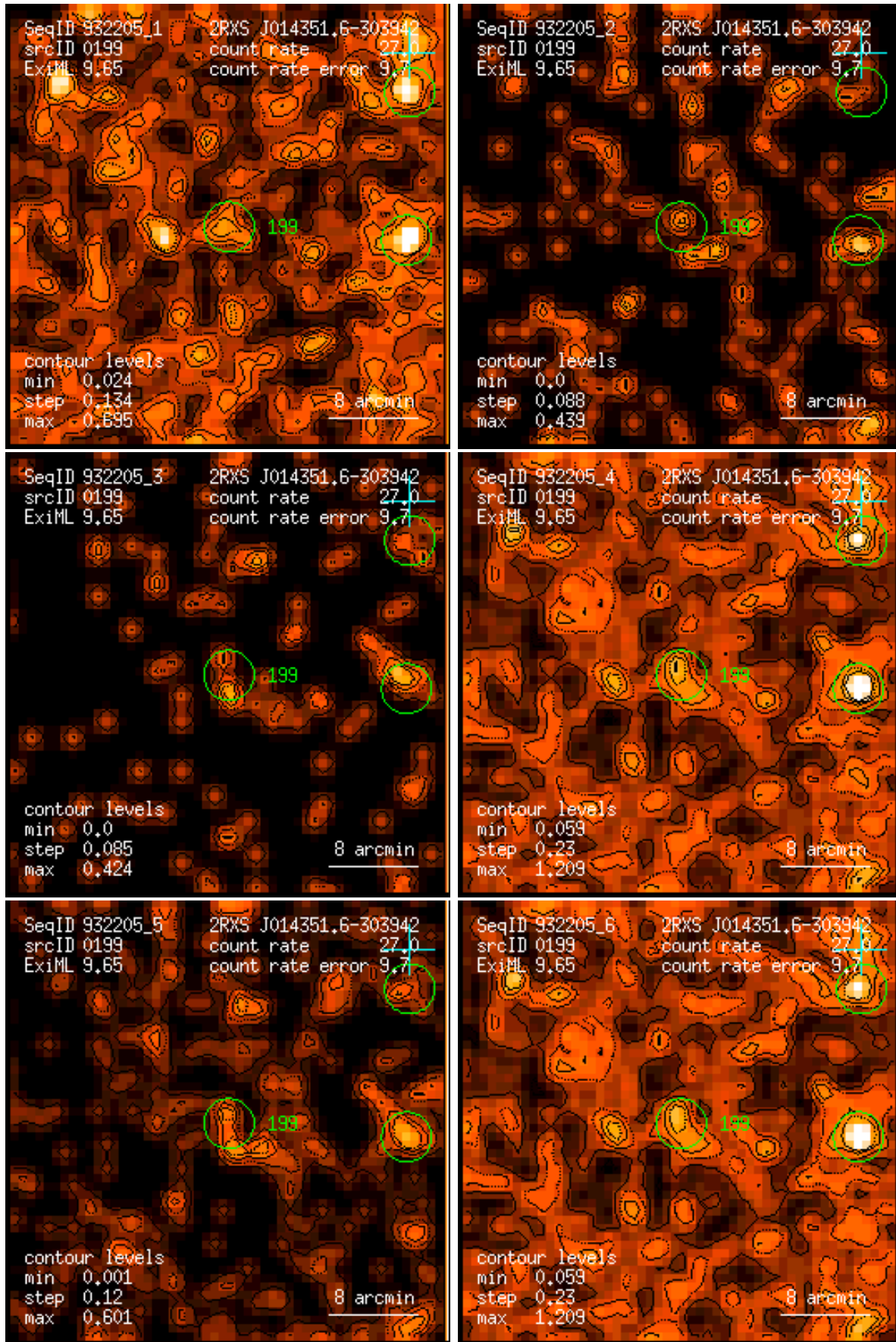
Figure 199: RASS 932205: detection 0199: band rate images, Gaussian filter: (1) PSPC channels 11 – 41, (2) 52 – 90, (3) 91 – 201, (4) 11 – 235, (5) 52 – 201, (6) 11 – 201. Broad band rates in counts/ks. Band rate contour levels in counts/ks/arcmin 2 .
