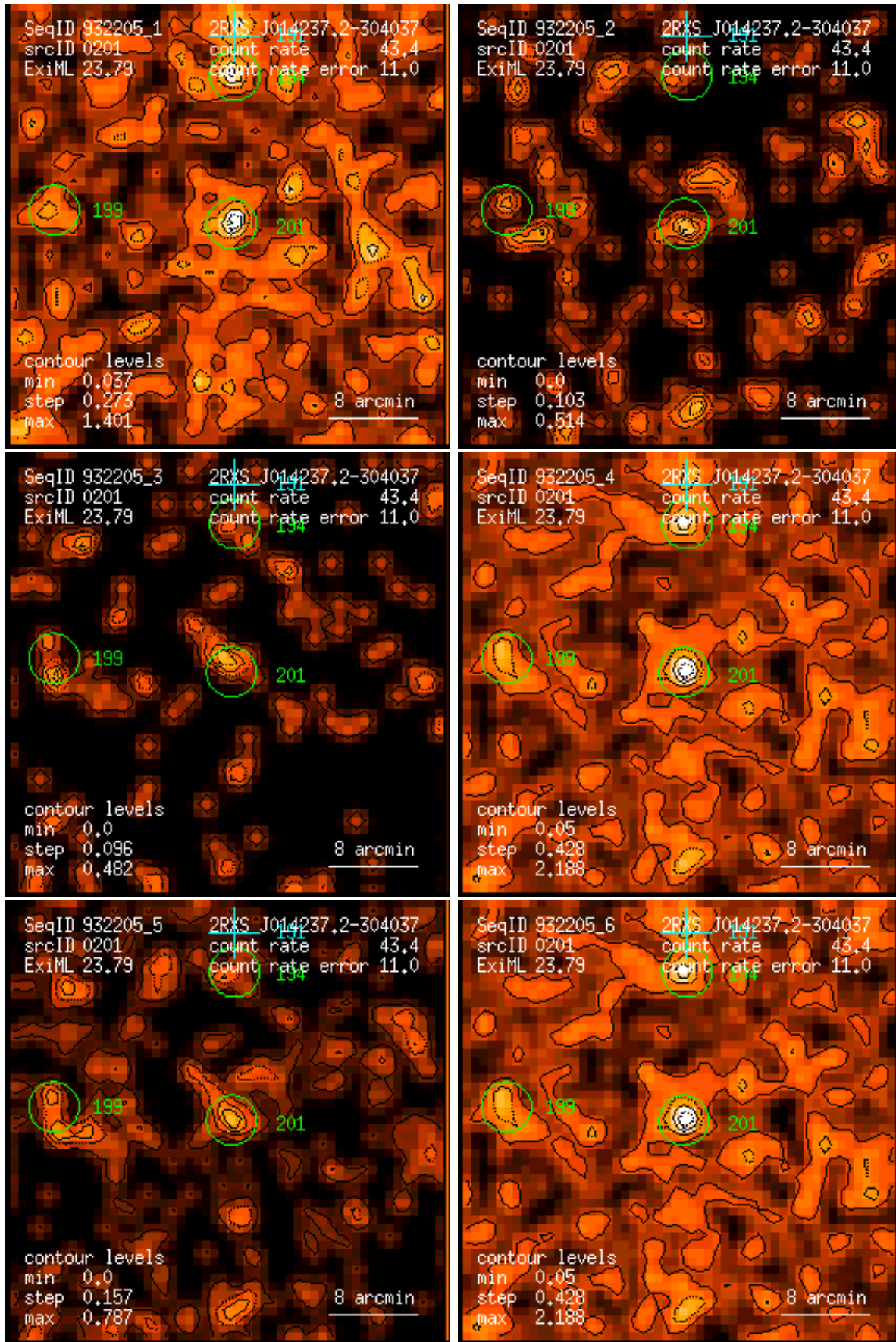
Figure 201: RASS 932205: detection 0201: band rate images, Gaussian filter: (1) PSPC channels 11 – 41, (2) 52 – 90, (3) 91 – 201, (4) 11 – 235, (5) 52 – 201, (6) 11 – 201. Broad band rates in counts/ks. Band rate contour levels in counts/ks/arcmin 2 .
