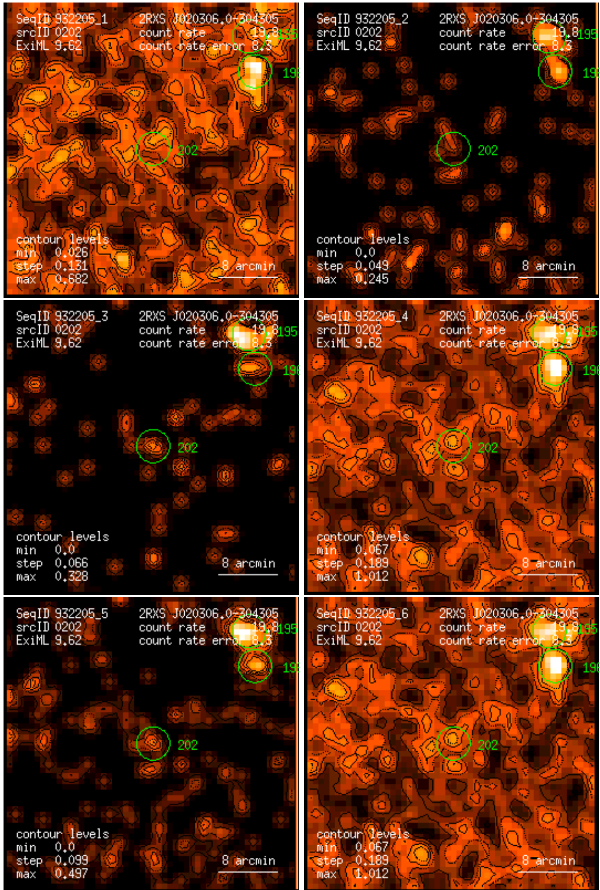
Figure 202: RASS 932205: detection 0202: band rate images, Gaussian filter: (1) PSPC channels 11 – 41, (2) 52 – 90, (3) 91 – 201, (4) 11 – 235, (5) 52 – 201, (6) 11 – 201. Broad band rates in counts/ks. Band rate contour levels in counts/ks/arcmin 2 .
