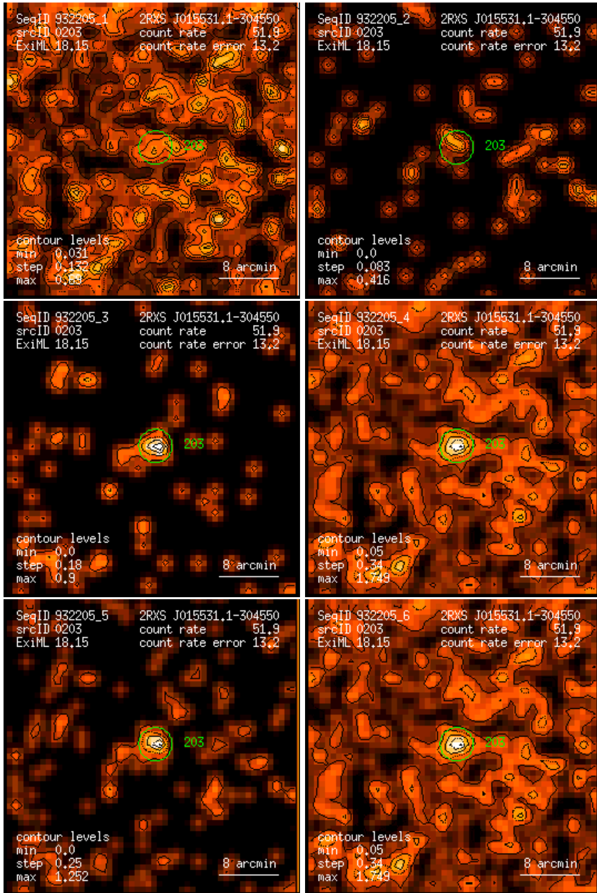
Figure 203: RASS 932205: detection 0203: band rate images, Gaussian filter: (1) PSPC channels 11 – 41, (2) 52 – 90, (3) 91 – 201, (4) 11 – 235, (5) 52 – 201, (6) 11 – 201. Broad band rates in counts/ks. Band rate contour levels in counts/ks/arcmin 2 .
