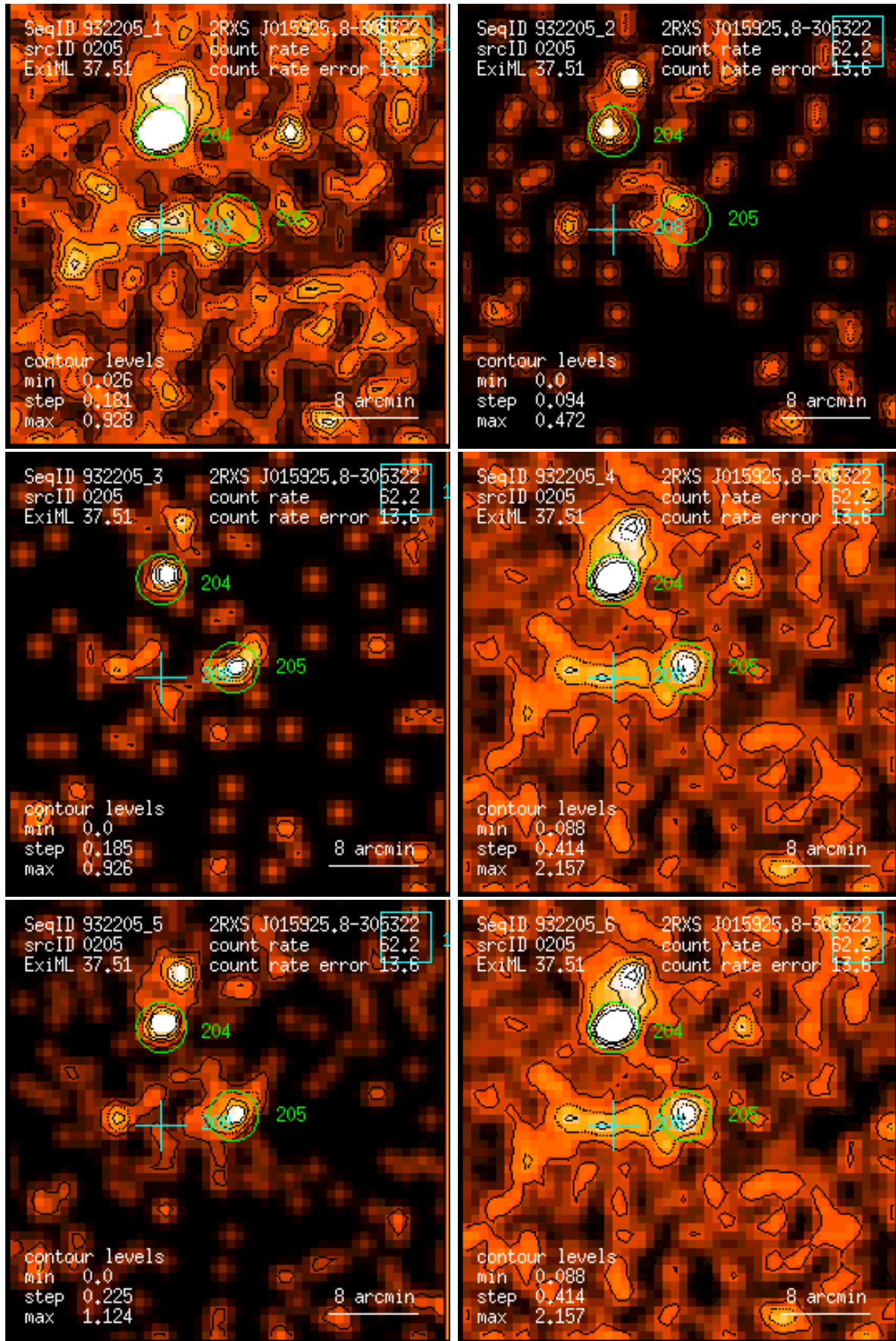
Figure 205: RASS 932205: detection 0205: band rate images, Gaussian filter: (1) PSPC channels 11 – 41, (2) 52 – 90, (3) 91 – 201, (4) 11 – 235, (5) 52 – 201, (6) 11 – 201. Broad band rates in counts/ks. Band rate contour levels in counts/ks/arcmin 2 .
