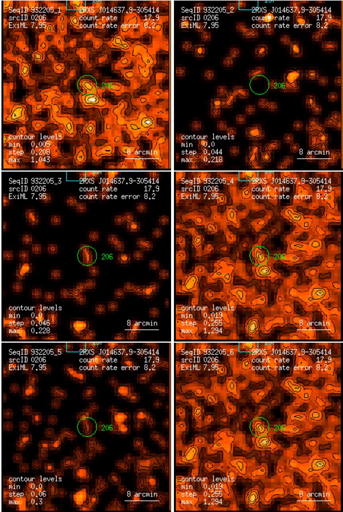
Figure 206: RASS 932205: detection 0206: band rate images, Gaussian filter: (1) PSPC channels 11 – 41, (2) 52 – 90, (3) 91 – 201, (4) 11 – 235, (5) 52 – 201, (6) 11 – 201. Broad band rates in counts/ks. Band rate contour levels in counts/ks/arcmin 2 .
