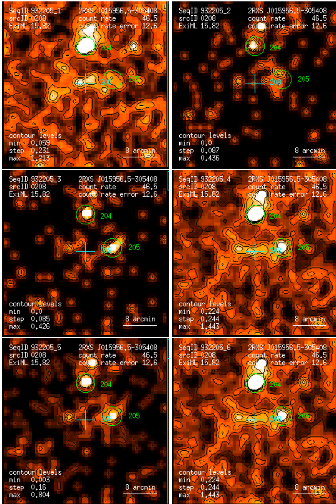
Figure 208: RASS 932205: detection 0208: band rate images, Gaussian filter: (1) PSPC channels 11 – 41, (2) 52 – 90, (3) 91 – 201, (4) 11 – 235, (5) 52 – 201, (6) 11 – 201. Broad band rates in counts/ks. Band rate contour levels in counts/ks/arcmin 2 .
