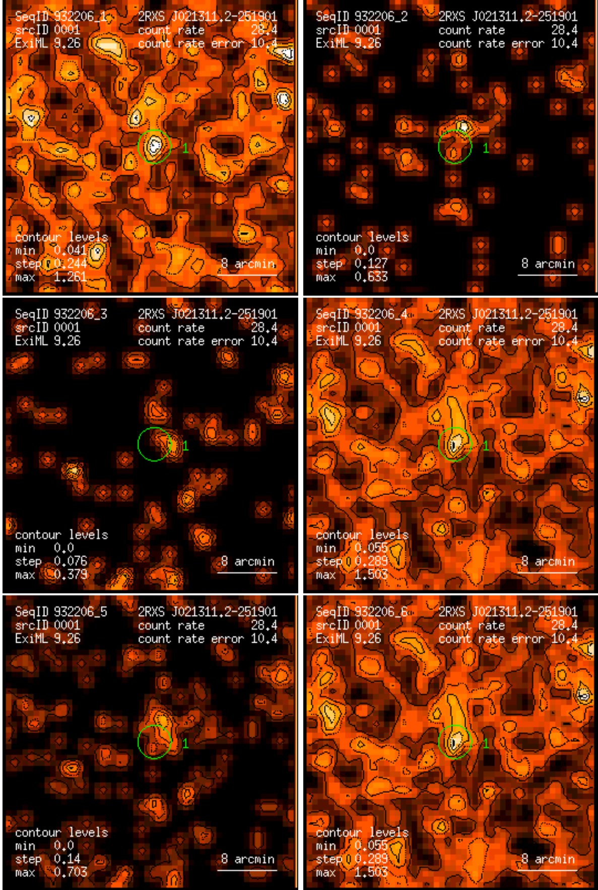
Figure 1: RASS 932206: detection 0001: band rate images, Gaussian filter: (1) PSPC channels 11 – 41, (2) 52 – 90, (3) 91 – 201, (4) 11 – 235, (5) 52 – 201, (6) 11 – 201. Broad band rates in counts/ks. Band rate contour levels in counts/ks/arcmin 2 .
