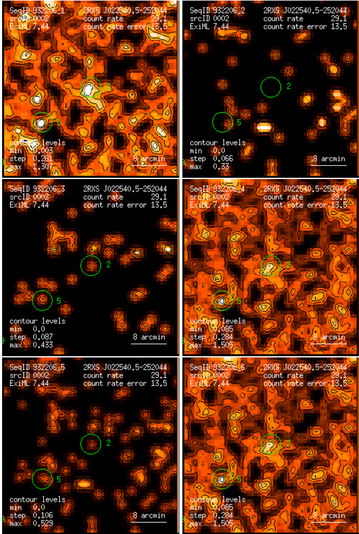
Figure 2: RASS 932206: detection 0002: band rate images, Gaussian filter: (1) PSPC channels 11 – 41, (2) 52 – 90, (3) 91 – 201, (4) 11 – 235, (5) 52 – 201, (6) 11 – 201. Broad band rates in counts/ks. Band rate contour levels in counts/ks/arcmin 2 .
