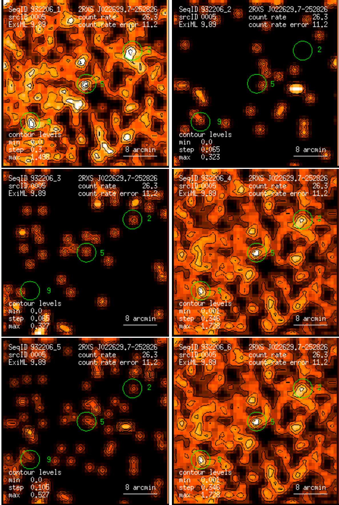
Figure 5: RASS 932206: detection 0005: band rate images, Gaussian filter: (1) PSPC channels 11 – 41, (2) 52 – 90, (3) 91 – 201, (4) 11 – 235, (5) 52 – 201, (6) 11 – 201. Broad band rates in counts/ks. Band rate contour levels in counts/ks/arcmin 2 .
