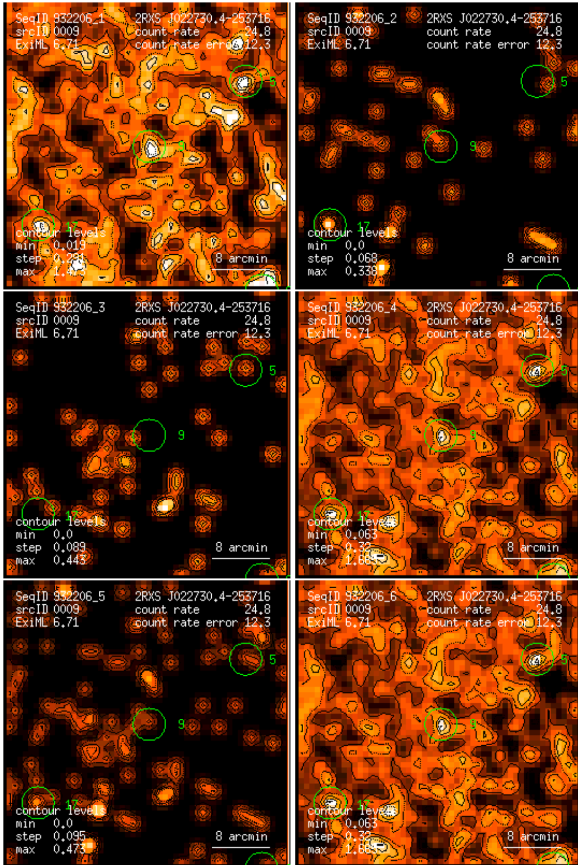
Figure 9: RASS 932206: detection 0009: band rate images, Gaussian filter: (1) PSPC channels 11 – 41, (2) 52 – 90, (3) 91 – 201, (4) 11 – 235, (5) 52 – 201, (6) 11 – 201. Broad band rates in counts/ks. Band rate contour levels in counts/ks/arcmin 2 .
