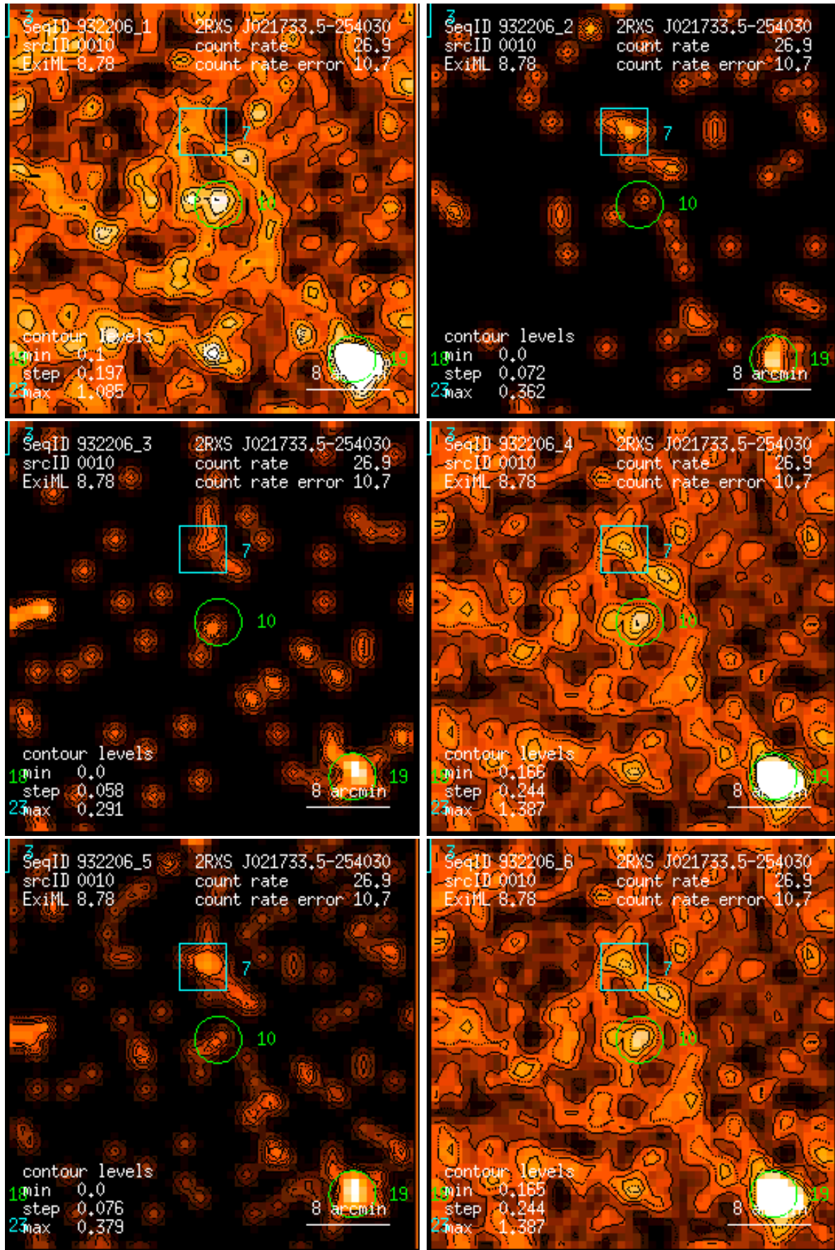
Figure 10: RASS 932206: detection 0010: band rate images, Gaussian filter: (1) PSPC channels 11 – 41, (2) 52 – 90, (3) 91 – 201, (4) 11 – 235, (5) 52 – 201, (6) 11 – 201. Broad band rates in counts/ks. Band rate contour levels in counts/ks/arcmin 2 .
