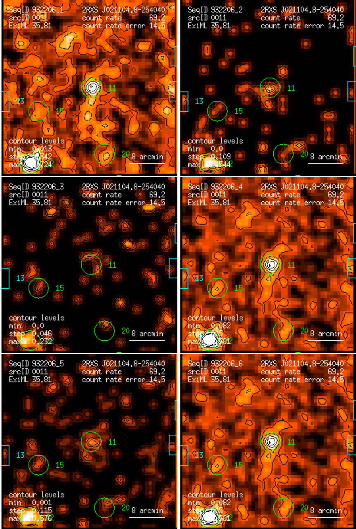
Figure 11: RASS 932206: detection 0011: band rate images, Gaussian filter: (1) PSPC channels 11 – 41, (2) 52 – 90, (3) 91 – 201, (4) 11 – 235, (5) 52 – 201, (6) 11 – 201. Broad band rates in counts/ks. Band rate contour levels in counts/ks/arcmin 2 .
