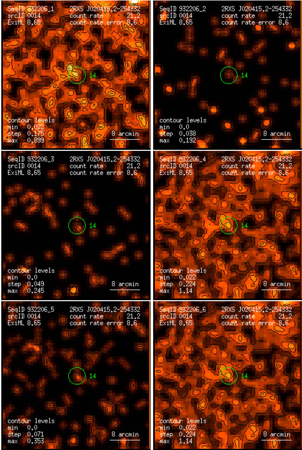
Figure 14: RASS 932206: detection 0014: band rate images, Gaussian filter: (1) PSPC channels 11 – 41, (2) 52 – 90, (3) 91 – 201, (4) 11 – 235, (5) 52 – 201, (6) 11 – 201. Broad band rates in counts/ks. Band rate contour levels in counts/ks/arcmin 2 .
