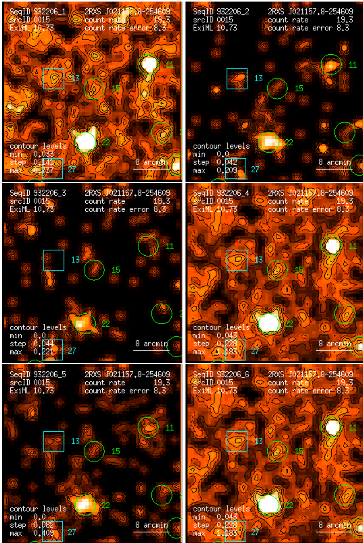
Figure 15: RASS 932206: detection 0015: band rate images, Gaussian filter: (1) PSPC channels 11 – 41, (2) 52 – 90, (3) 91 – 201, (4) 11 – 235, (5) 52 – 201, (6) 11 – 201. Broad band rates in counts/ks. Band rate contour levels in counts/ks/arcmin 2 .
