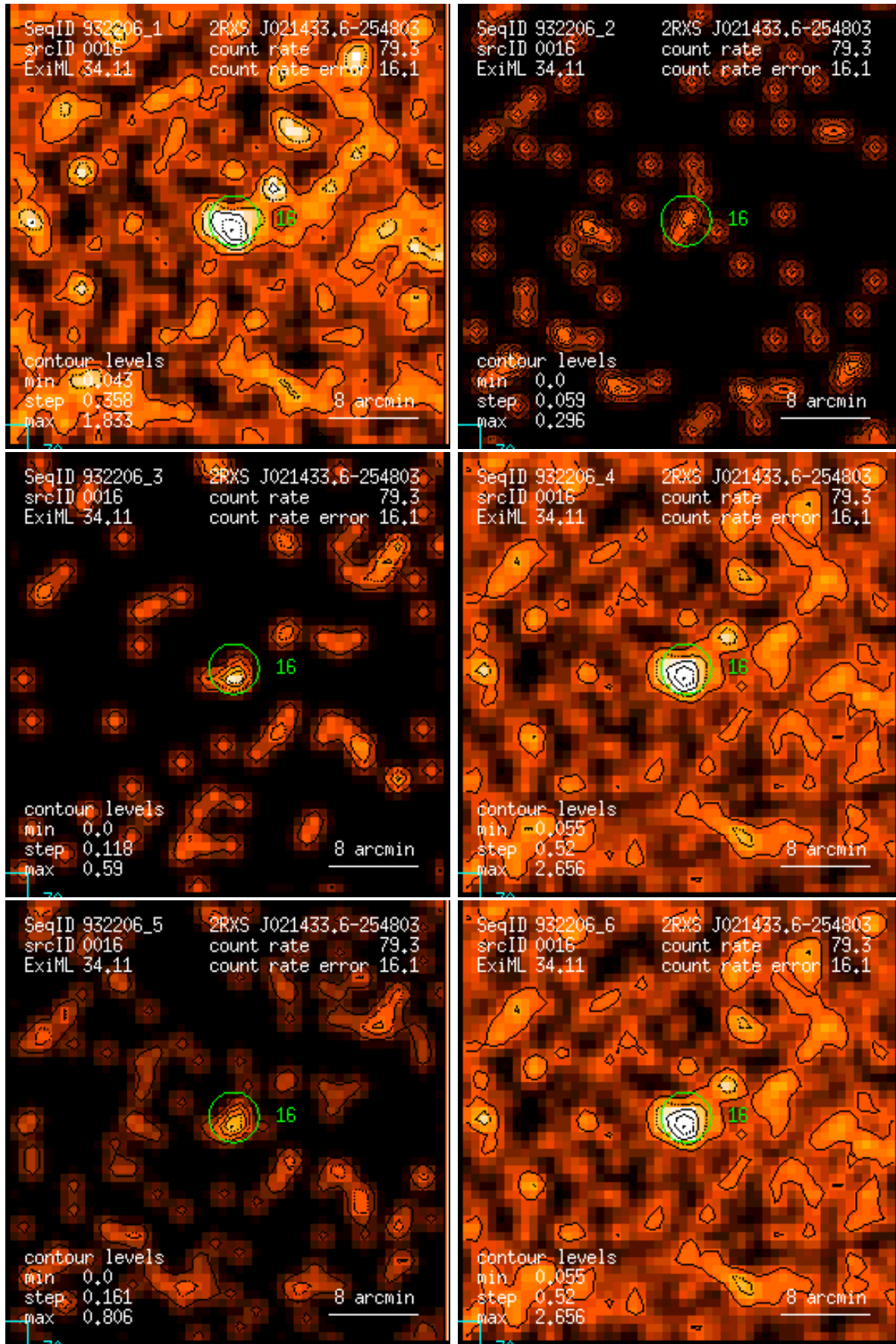
Figure 16: RASS 932206: detection 0016: band rate images, Gaussian filter: (1) PSPC channels 11 – 41, (2) 52 – 90, (3) 91 – 201, (4) 11 – 235, (5) 52 – 201, (6) 11 – 201. Broad band rates in counts/ks. Band rate contour levels in counts/ks/arcmin 2 .
