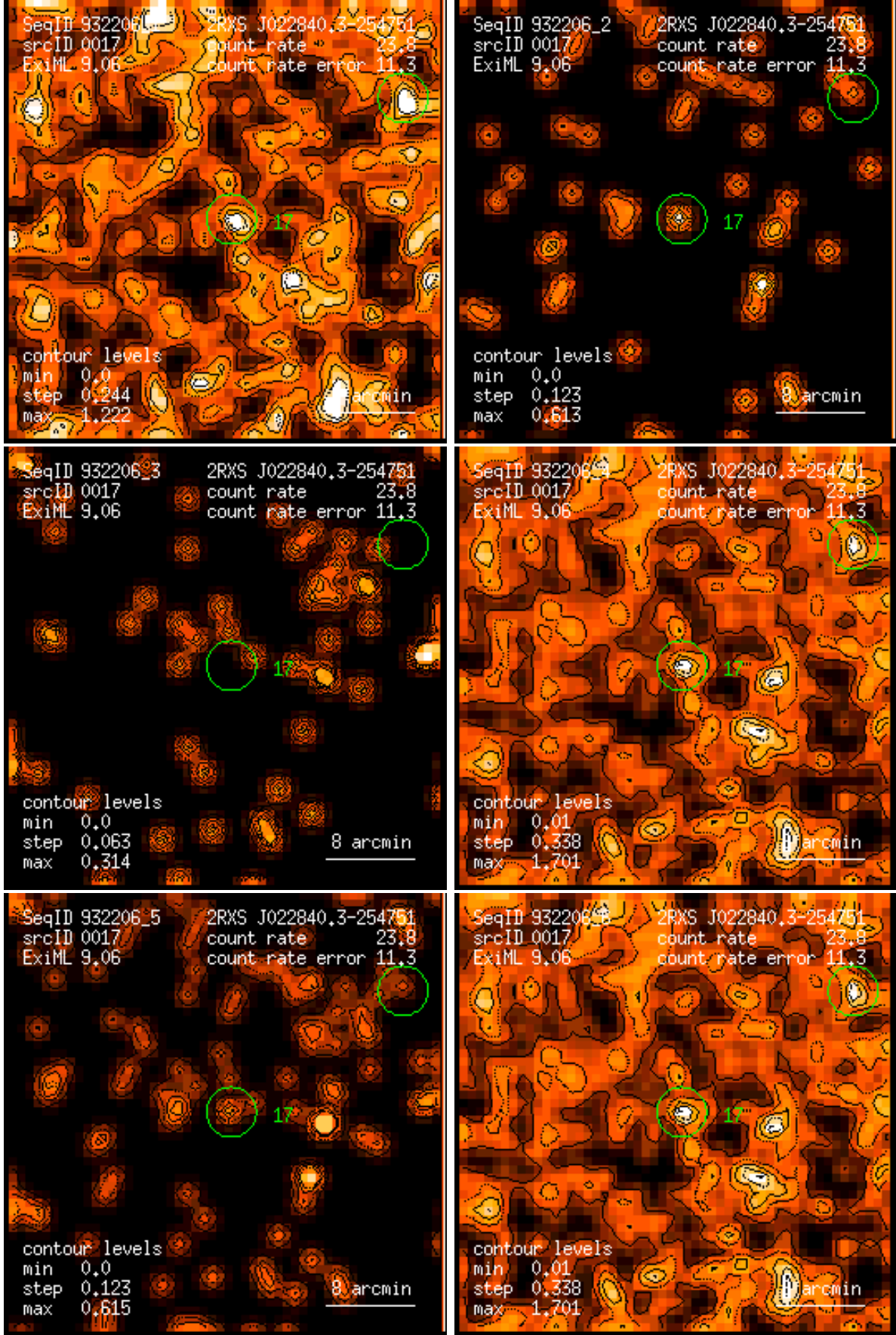
Figure 17: RASS 932206: detection 0017: band rate images, Gaussian filter: (1) PSPC channels 11 – 41, (2) 52 – 90, (3) 91 – 201, (4) 11 – 235, (5) 52 – 201, (6) 11 – 201. Broad band rates in counts/ks. Band rate contour levels in counts/ks/arcmin 2 .
