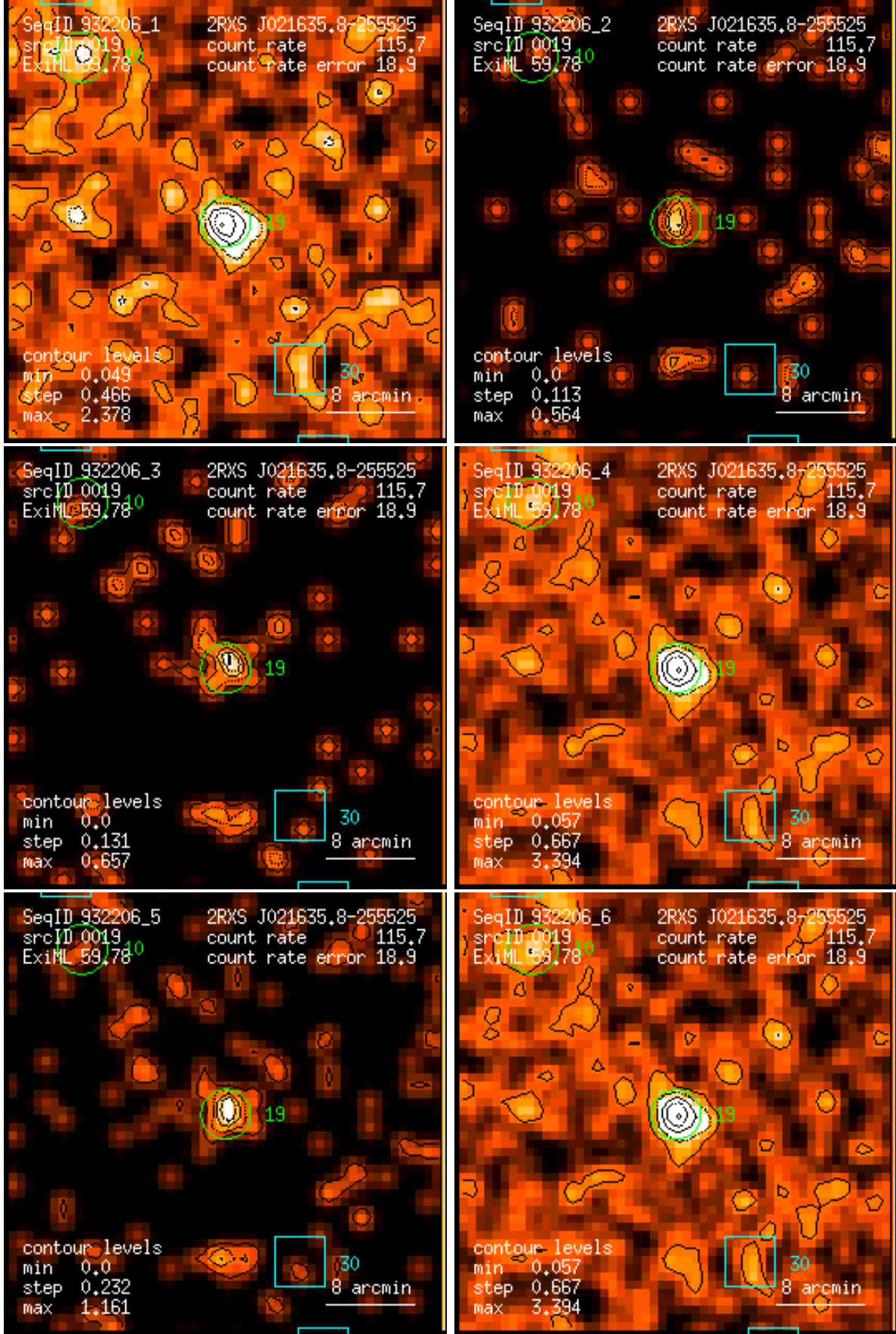
Figure 19: RASS 932206: detection 0019: band rate images, Gaussian filter: (1) PSPC channels 11 – 41, (2) 52 – 90, (3) 91 – 201, (4) 11 – 235, (5) 52 – 201, (6) 11 – 201. Broad band rates in counts/ks. Band rate contour levels in counts/ks/arcmin 2 .
