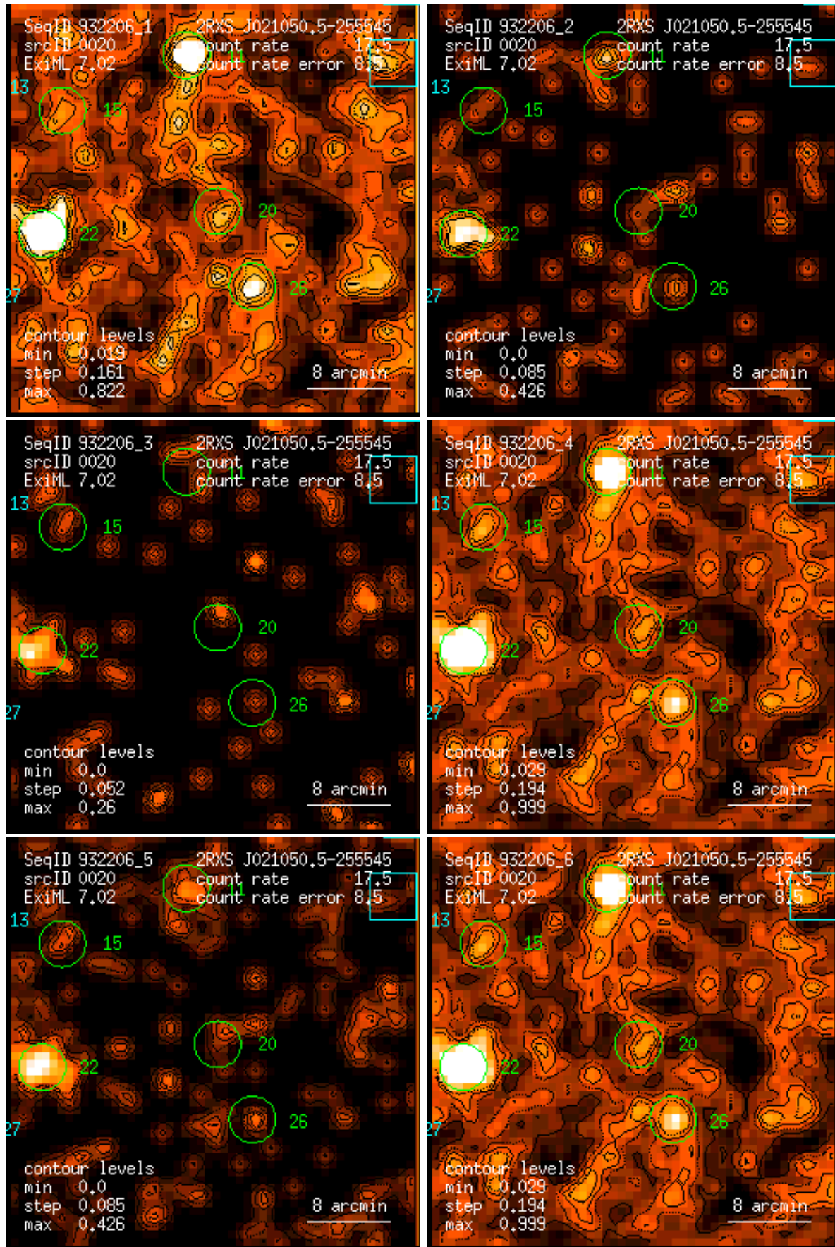
Figure 20: RASS 932206: detection 0020: band rate images, Gaussian filter: (1) PSPC channels 11 – 41, (2) 52 – 90, (3) 91 – 201, (4) 11 – 235, (5) 52 – 201, (6) 11 – 201. Broad band rates in counts/ks. Band rate contour levels in counts/ks/arcmin 2 .
