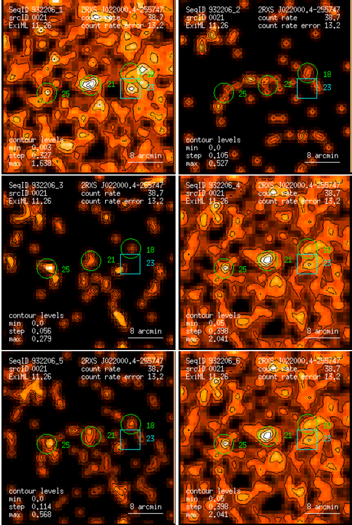
Figure 21: RASS 932206: detection 0021: band rate images, Gaussian filter: (1) PSPP channels 11 – 41, (2) 52 – 90, (3) 91 – 201, (4) 11 – 235, (5) 52 – 201, (6) 11 – 201. Broad band rates in counts/ks. Band rate contour levels in counts/ks/arcmin 2 .
