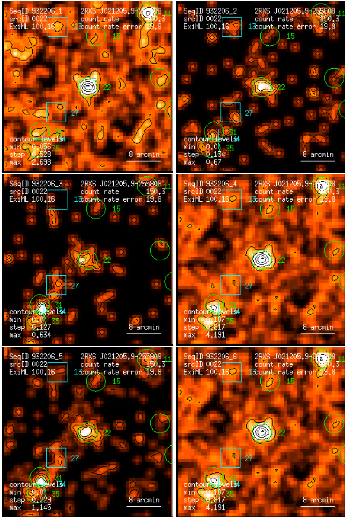
Figure 22: RASS 932206: detection 0022: band rate images, Gaussian filter: (1) PSPC channels 11 – 41, (2) 52 – 90, (3) 91 – 201, (4) 11 – 235, (5) 52 – 201, (6) 11 – 201. Broad band rates in counts/ks. Band rate contour levels in counts/ks/arcmin 2 .
