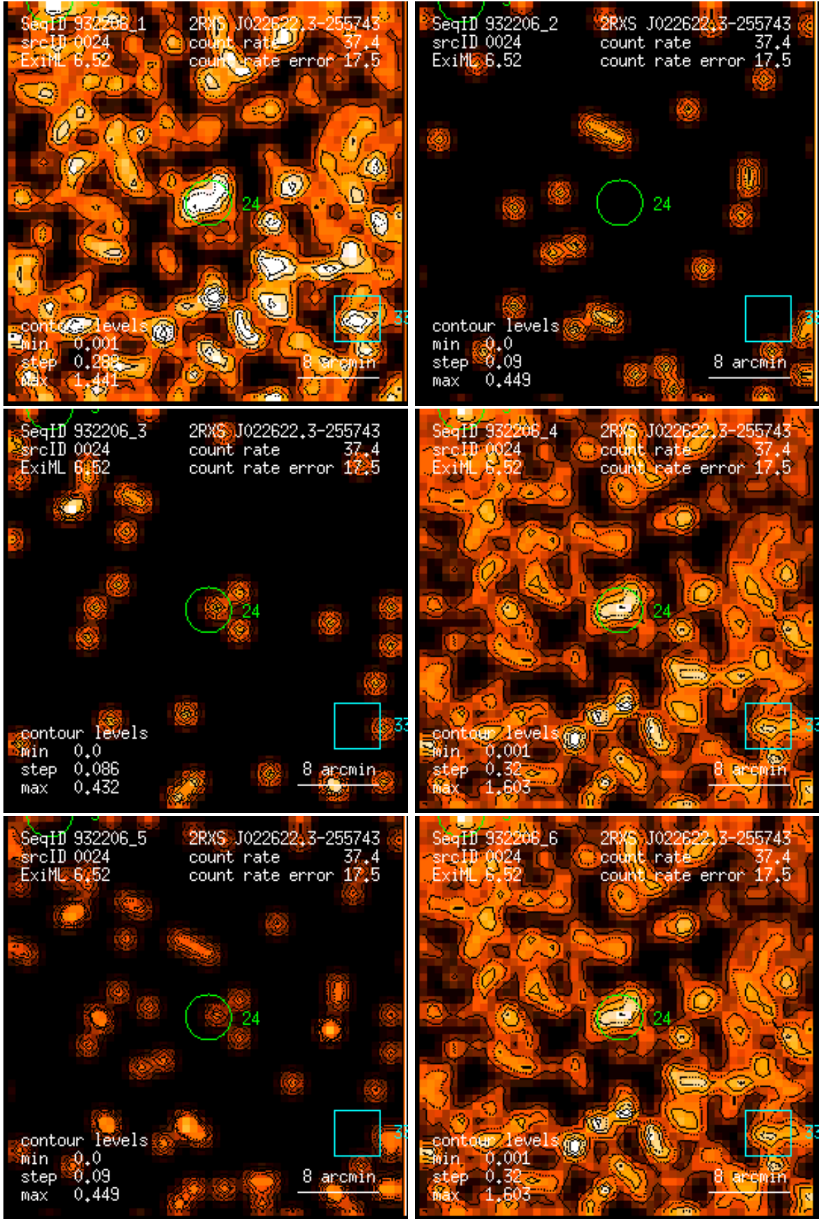
Figure 24: RASS 932206: detection 0024: band rate images, Gaussian filter: (1) PSPC channels 11 – 41, (2) 52 – 90, (3) 91 – 201, (4) 11 – 235, (5) 52 – 201, (6) 11 – 201. Broad band rates in counts/ks. Band rate contour levels in counts/ks/arcmin 2 .
