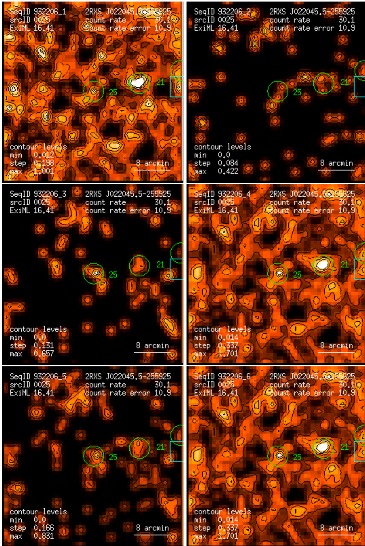
Figure 25: RASS 932206: detection 0025: band rate images, Gaussian filter: (1) PSPC channels 11 – 41, (2) 52 – 90, (3) 91 – 201, (4) 11 – 235, (5) 52 – 201, (6) 11 – 201. Broad band rates in counts/ks. Band rate contour levels in counts/ks/arcmin 2 .
