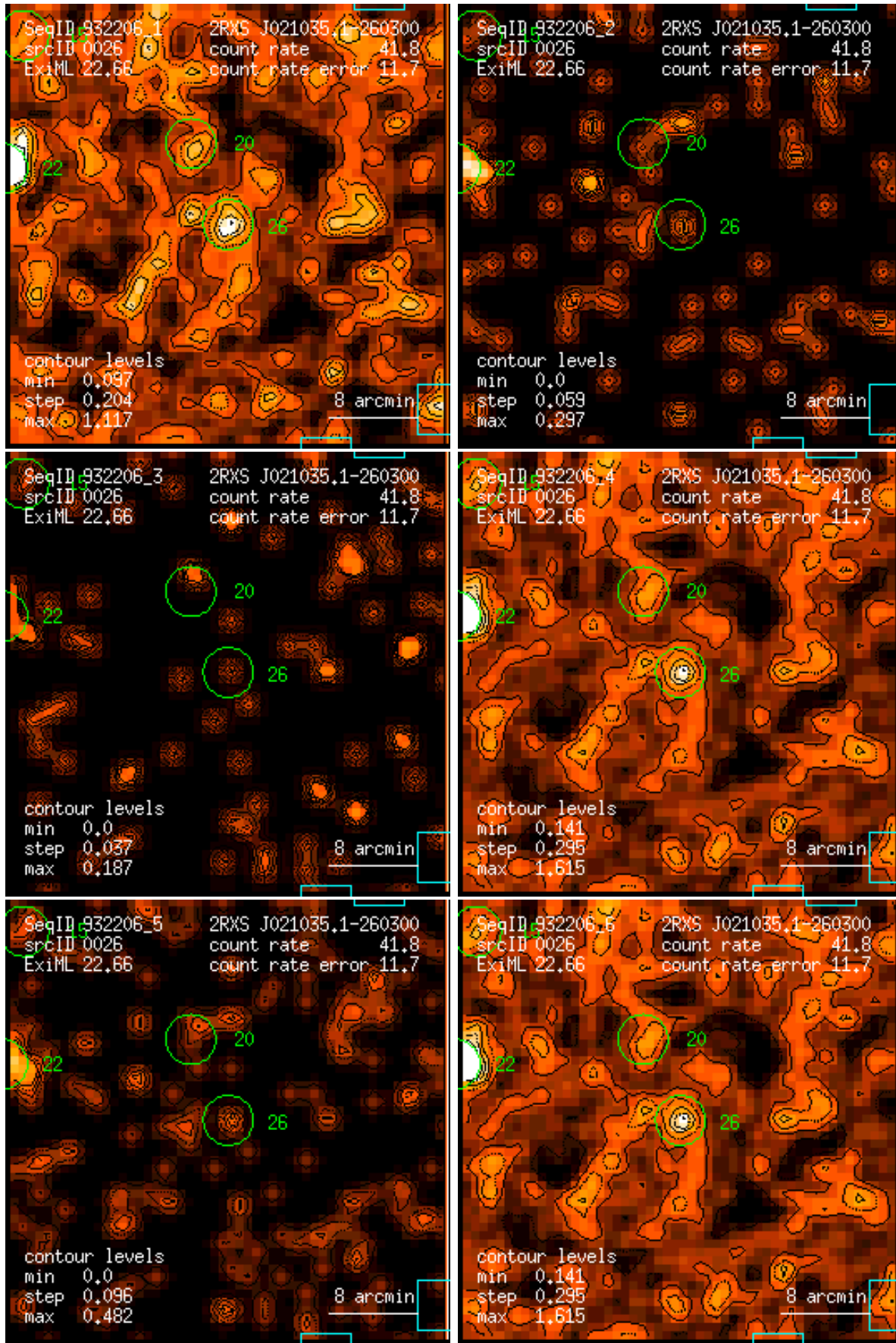
Figure 26: RASS 932206: detection 0026: band rate images, Gaussian filter: (1) PSPC channels 11 – 41, (2) 52 – 90, (3) 91 – 201, (4) 11 – 235, (5) 52 – 201, (6) 11 – 201. Broad band rates in counts/ks. Band rate contour levels in counts/ks/arcmin 2 .
