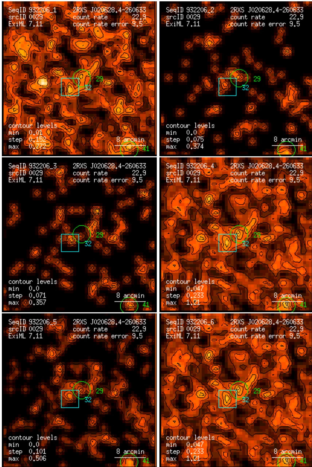
Figure 29: RASS 932206: detection 0029: band rate images, Gaussian filter: (1) PSPC channels 11 – 41, (2) 52 – 90, (3) 91 – 201, (4) 11 – 235, (5) 52 – 201, (6) 11 – 201. Broad band rates in counts/ks. Band rate contour levels in counts/ks/arcmin 2 .
