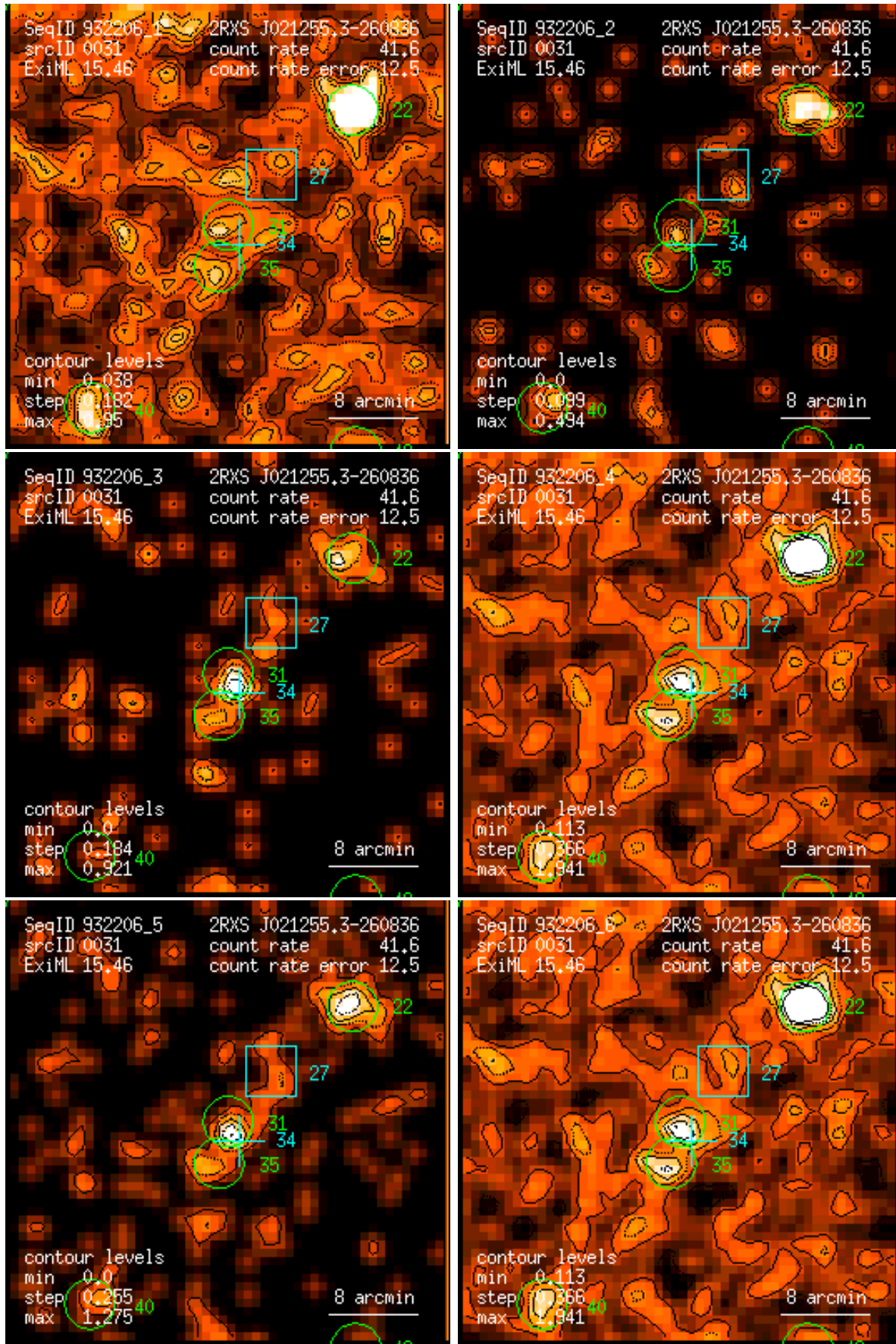
Figure 31: RASS 932206: detection 0031: band rate images, Gaussian filter: (1) PSPC channels 11 – 41, (2) 52 – 90, (3) 91 – 201, (4) 11 – 235, (5) 52 – 201, (6) 11 – 201. Broad band rates in counts/ks. Band rate contour levels in counts/ks/arcmin 2 .
