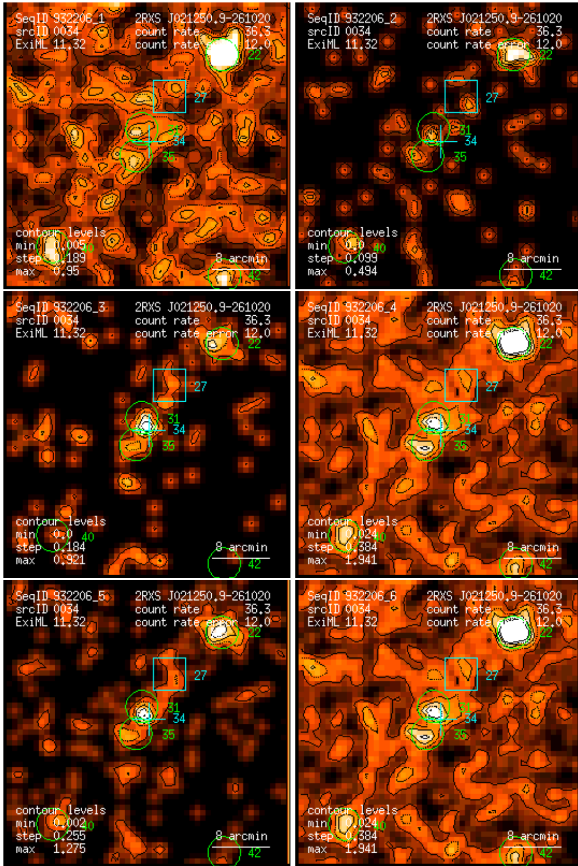
Figure 34: RASS 932206: detection 0034: band rate images, Gaussian filter: (1) PSPC channels 11 – 41, (2) 52 – 90, (3) 91 – 201, (4) 11 – 235, (5) 52 – 201, (6) 11 – 201. Broad band rates in counts/ks. Band rate contour levels in counts/ks/arcmin 2 .
