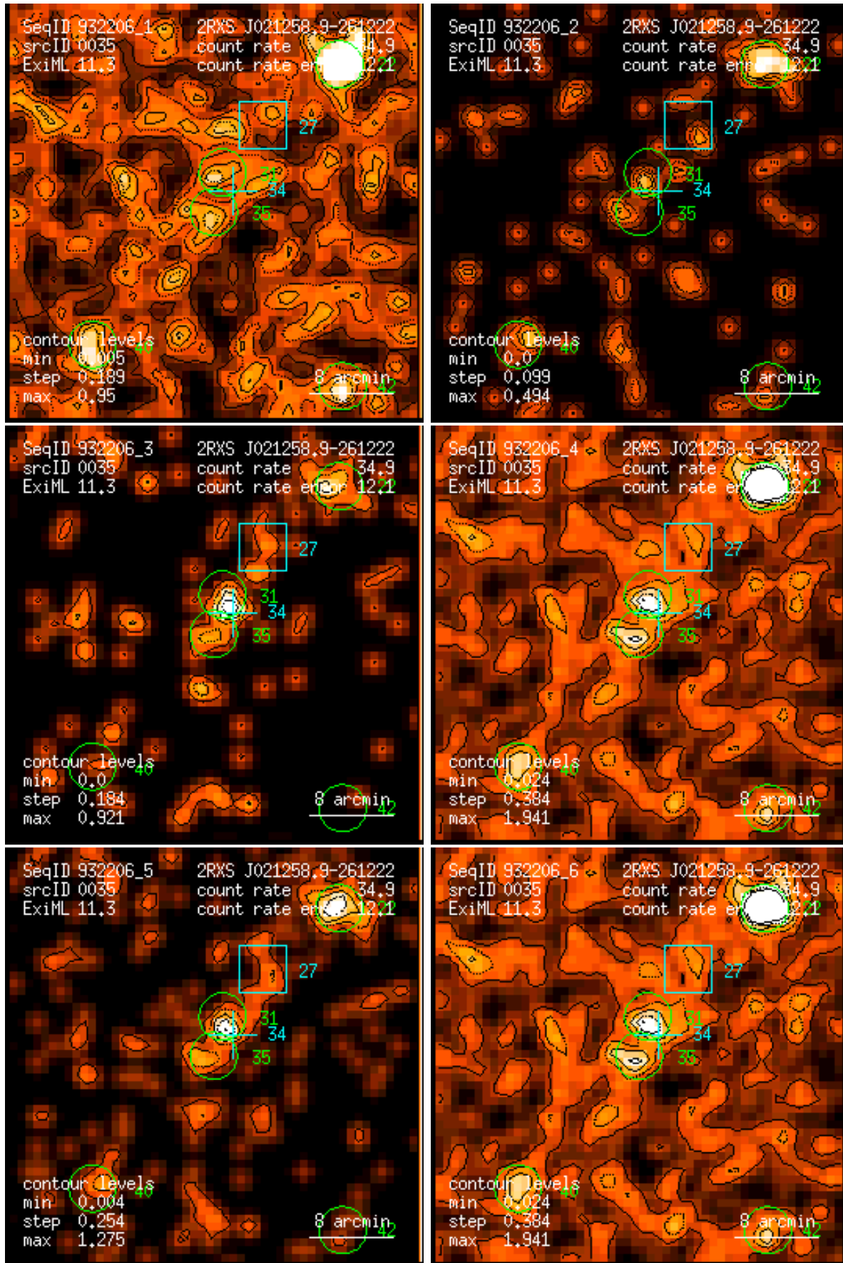
Figure 35: RASS 932206: detection 0035: band rate images, Gaussian filter: (1) PSPC channels 11 – 41, (2) 52 – 90, (3) 91 – 201, (4) 11 – 235, (5) 52 – 201, (6) 11 – 201. Broad band rates in counts/ks. Band rate contour levels in counts/ks/arcmin 2 .
