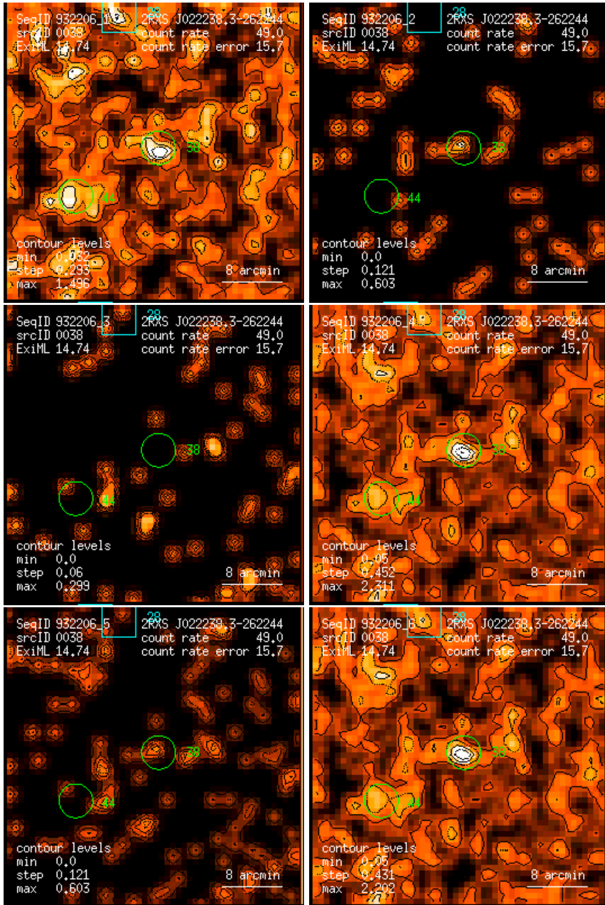
Figure 38: RASS 932206: detection 0038: band rate images, Gaussian filter: (1) PSPC channels 11 – 41, (2) 52 – 90, (3) 91 – 201, (4) 11 – 235, (5) 52 – 201, (6) 11 – 201. Broad band rates in counts/ks. Band rate contour levels in counts/ks/arcmin 2 .
