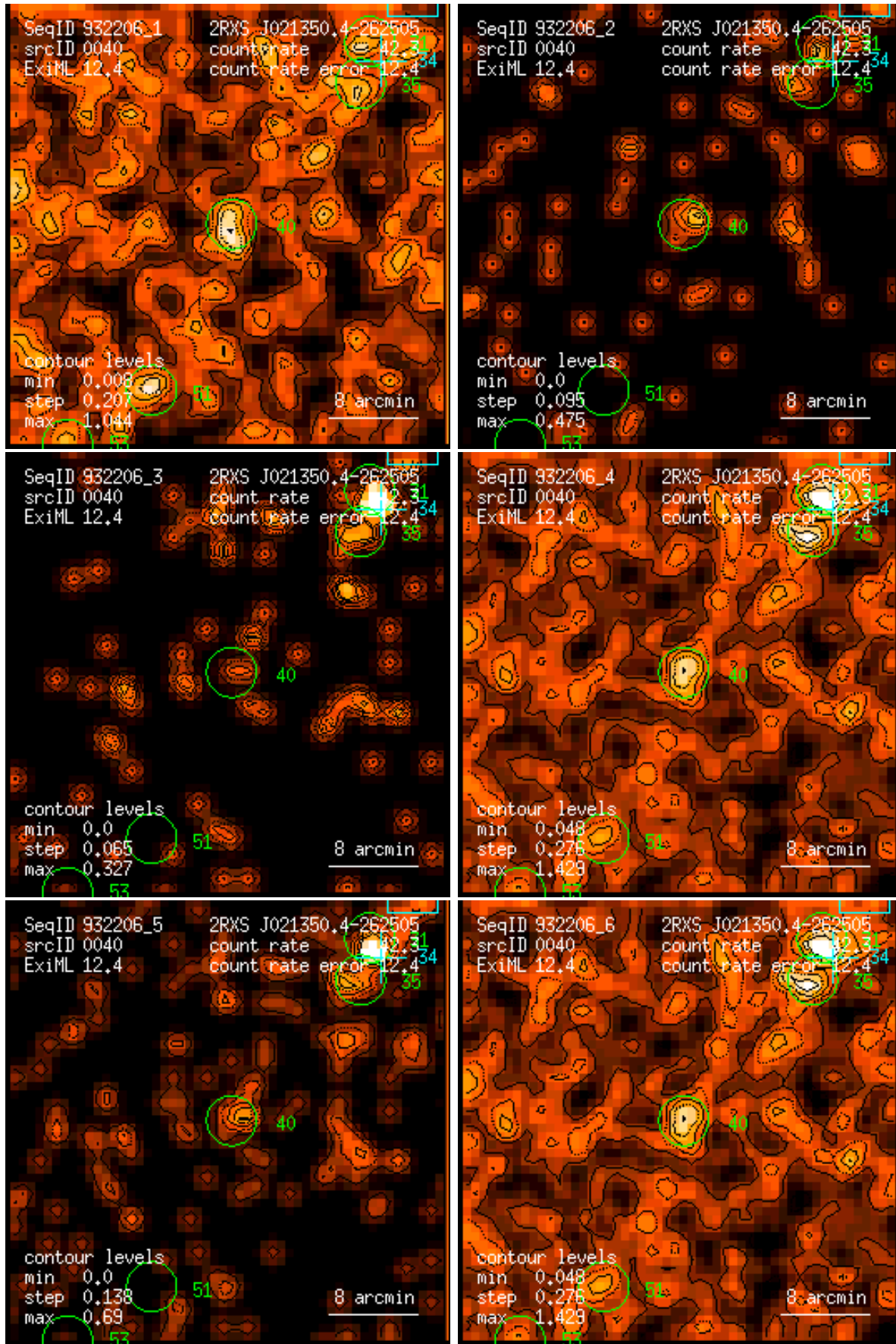
Figure 40: RASS 932206: detection 0040: band rate images, Gaussian filter: (1) PSPC channels 11 – 41, (2) 52 – 90, (3) 91 – 201, (4) 11 – 235, (5) 52 – 201, (6) 11 – 201. Broad band rates in counts/ks. Band rate contour levels in counts/ks/arcmin 2 .
