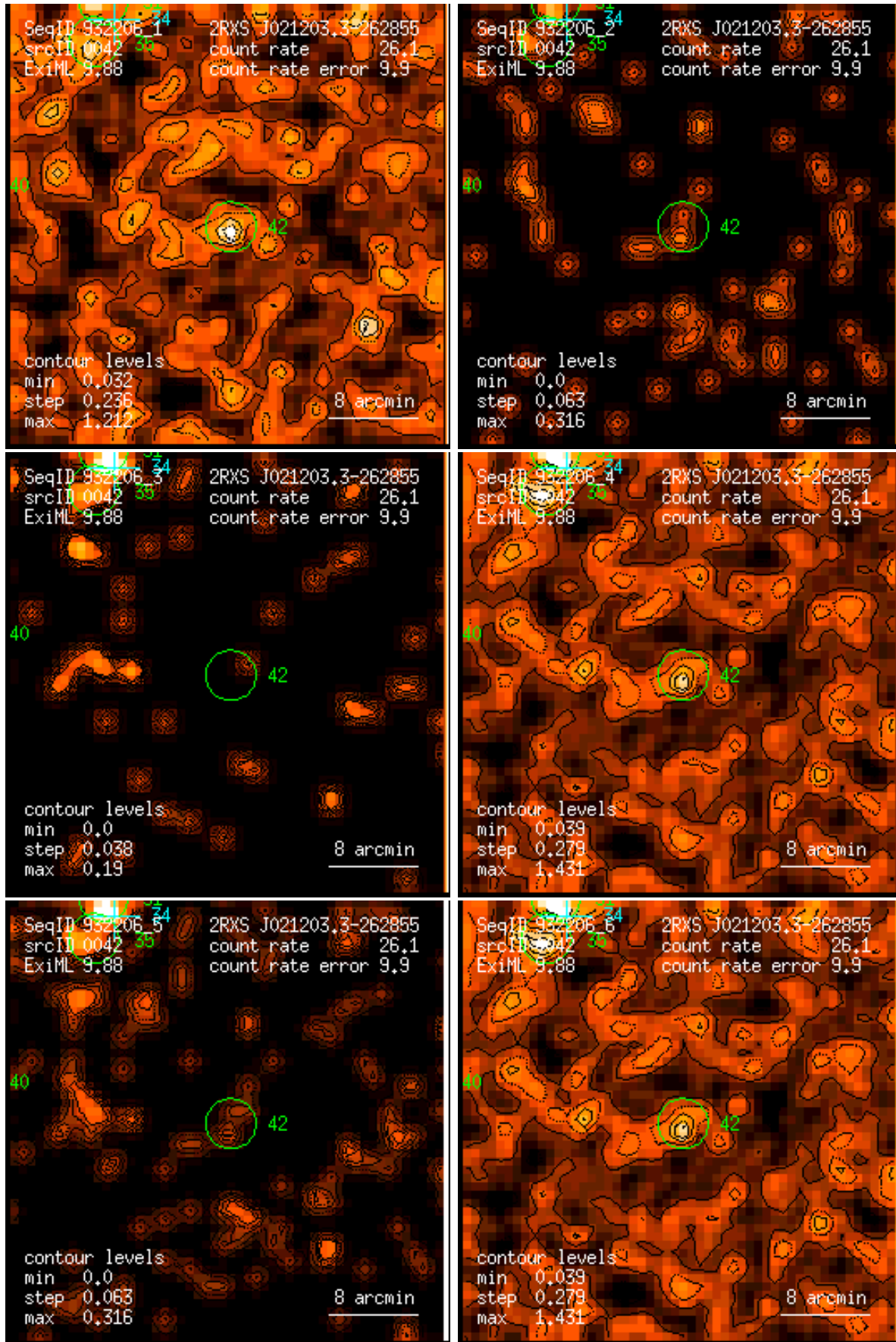
Figure 42: RASS 932206: detection 0042: band rate images, Gaussian filter: (1) PSPC channels 11 – 41, (2) 52 – 90, (3) 91 – 201, (4) 11 – 235, (5) 52 – 201, (6) 11 – 201. Broad band rates in counts/ks. Band rate contour levels in counts/ks/arcmin 2 .
