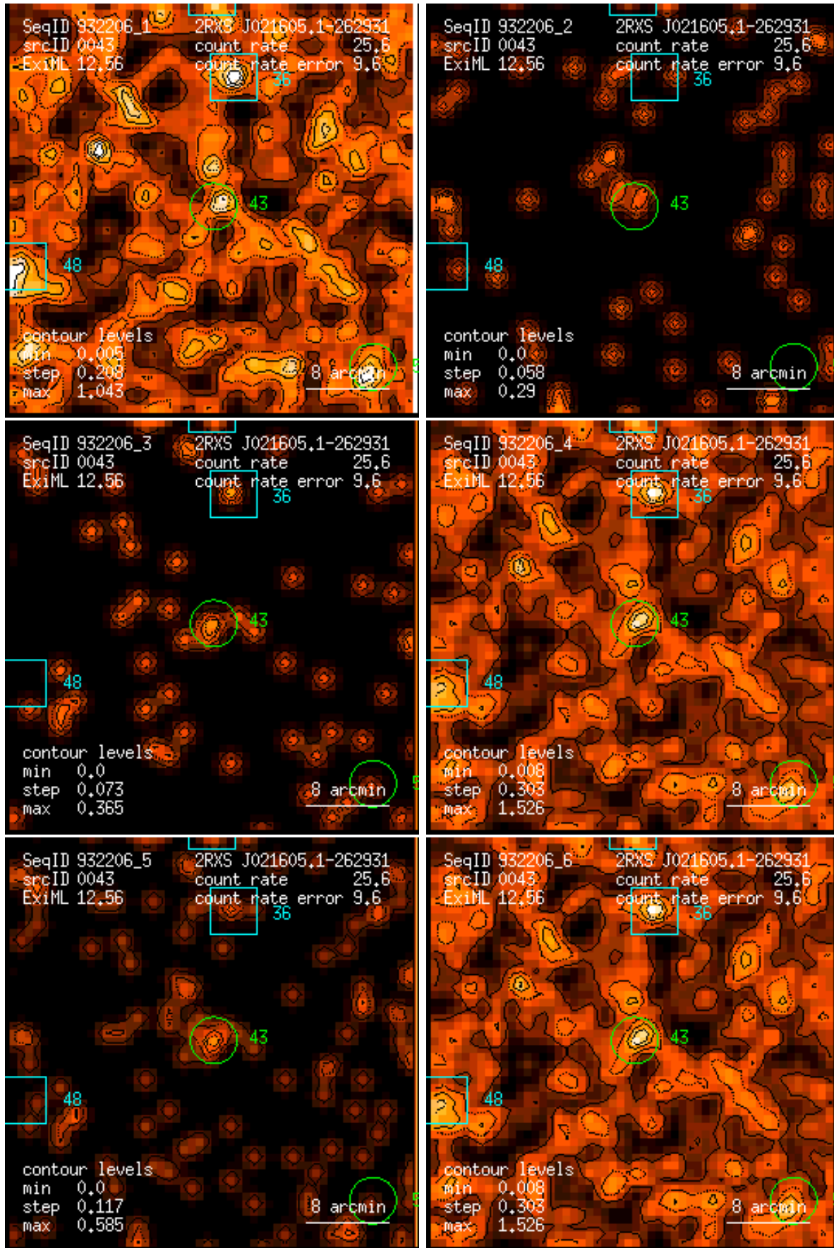
Figure 43: RASS 932206: detection 0043: band rate images, Gaussian filter: (1) PSPC channels 11 – 41, (2) 52 – 90, (3) 91 – 201, (4) 11 – 235, (5) 52 – 201, (6) 11 – 201. Broad band rates in counts/ks. Band rate contour levels in counts/ks/arcmin 2 .
