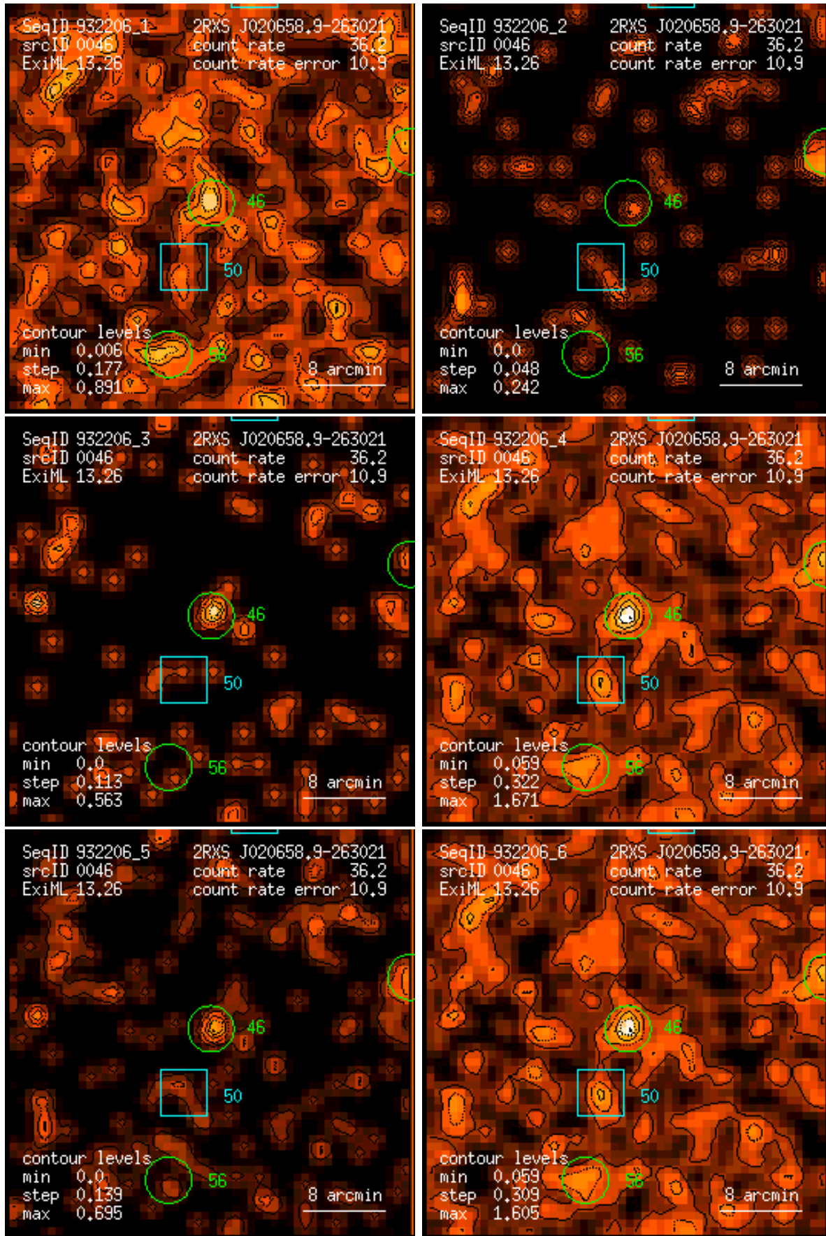
Figure 46: RASS 932206: detection 0046: band rate images, Gaussian filter: (1) PSPC channels 11 – 41, (2) 52 – 90, (3) 91 – 201, (4) 11 – 235, (5) 52 – 201, (6) 11 – 201. Broad band rates in counts/ks. Band rate contour levels in counts/ks/arcmin 2 .
