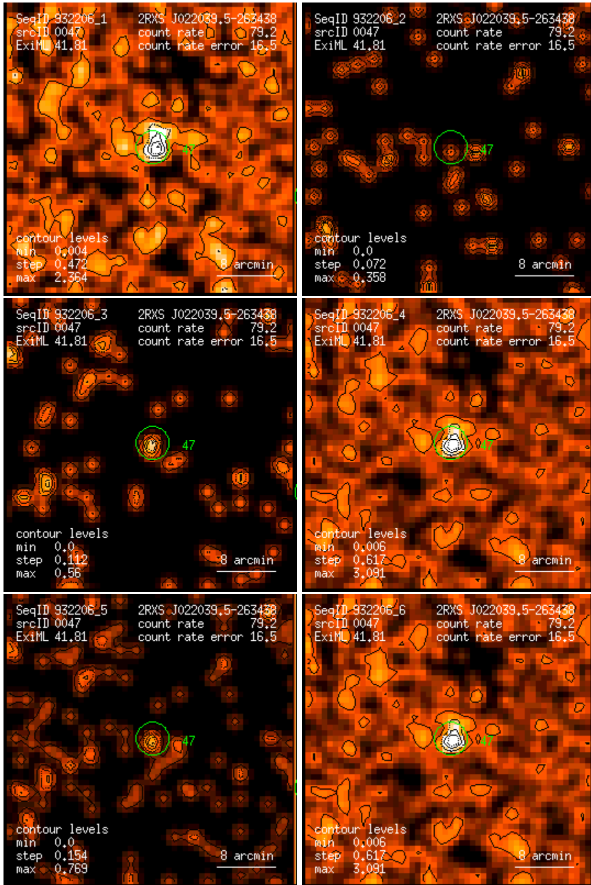
Figure 47: RASS 932206: detection 0047: band rate images, Gaussian filter: (1) PSPC channels 11 – 41, (2) 52 – 90, (3) 91 – 201, (4) 11 – 235, (5) 52 – 201, (6) 11 – 201. Broad band rates in counts/ks. Band rate contour levels in counts/ks/arcmin 2 .
