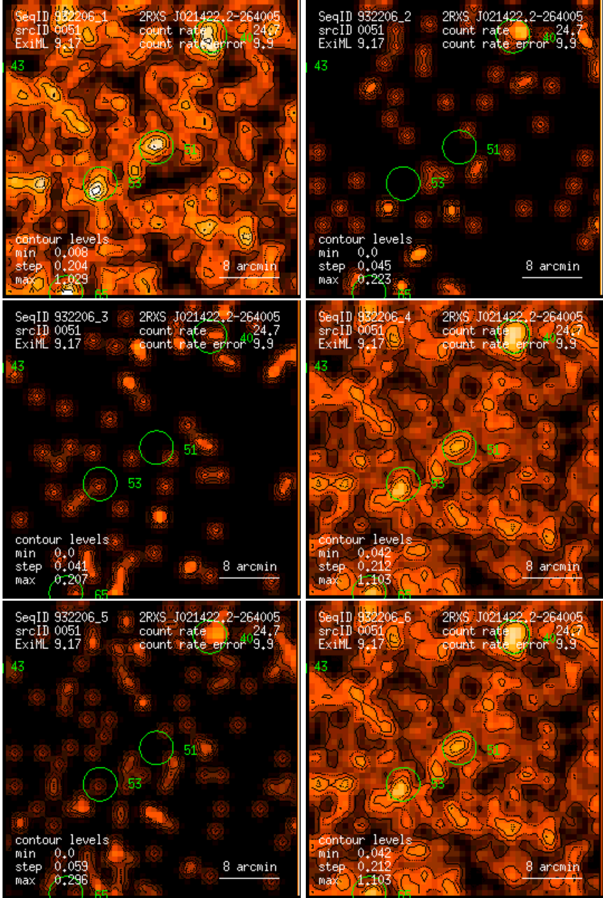
Figure 51: RASS 932206: detection 0051: band rate images, Gaussian filter: (1) PSPC channels 11 – 41, (2) 52 – 90, (3) 91 – 201, (4) 11 – 235, (5) 52 – 201, (6) 11 – 201. Broad band rates in counts/ks. Band rate contour levels in counts/ks/arcmin 2 .
