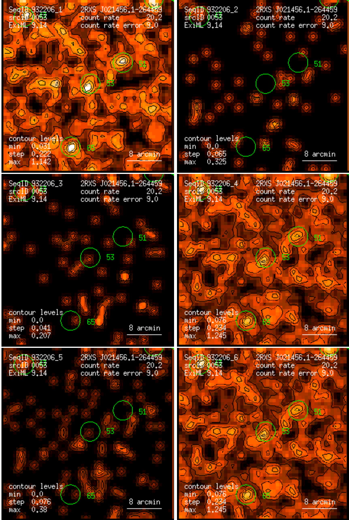
Figure 53: RASS 932206: detection 0053: band rate images, Gaussian filter: (1) PSPC channels 11 – 41, (2) 52 – 90, (3) 91 – 201, (4) 11 – 235, (5) 52 – 201, (6) 11 – 201. Broad band rates in counts/ks. Band rate contour levels in counts/ks/arcmin 2 .
