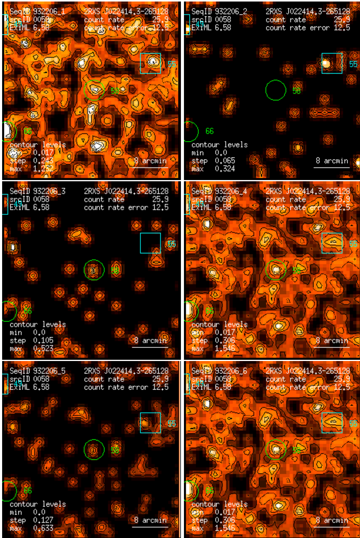
Figure 58: RASS 932206: detection 0058: band rate images, Gaussian filter: (1) PSPC channels 11 – 41, (2) 52 – 90, (3) 91 – 201, (4) 11 – 235, (5) 52 – 201, (6) 11 – 201. Broad band rates in counts/ks. Band rate contour levels in counts/ks/arcmin 2 .
