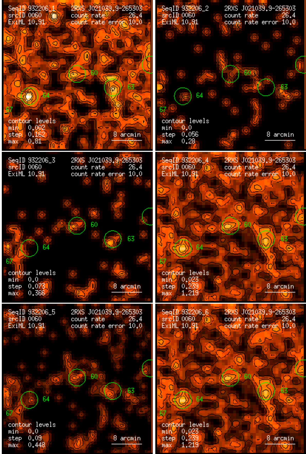
Figure 60: RASS 932206: detection 0060: band rate images, Gaussian filter: (1) PSPC channels 11 – 41, (2) 52 – 90, (3) 91 – 201, (4) 11 – 235, (5) 52 – 201, (6) 11 – 201. Broad band rates in counts/ks. Band rate contour levels in counts/ks/arcmin 2 .
