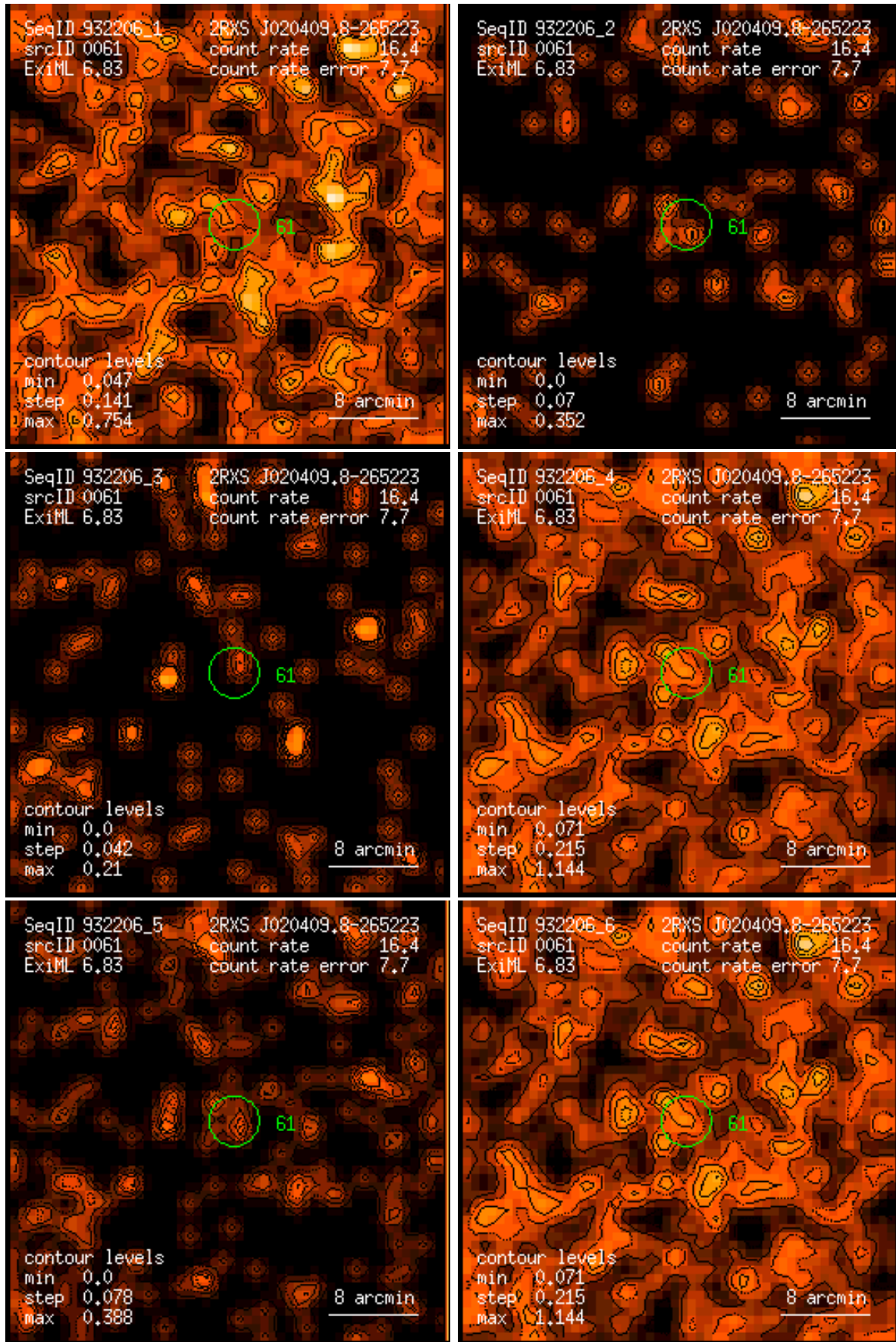
Figure 61: RASS 932206: detection 0061: band rate images, Gaussian filter: (1) PSPC channels 11 – 41, (2) 52 – 90, (3) 91 – 201, (4) 11 – 235, (5) 52 – 201, (6) 11 – 201. Broad band rates in counts/ks. Band rate contour levels in counts/ks/arcmin 2 .
