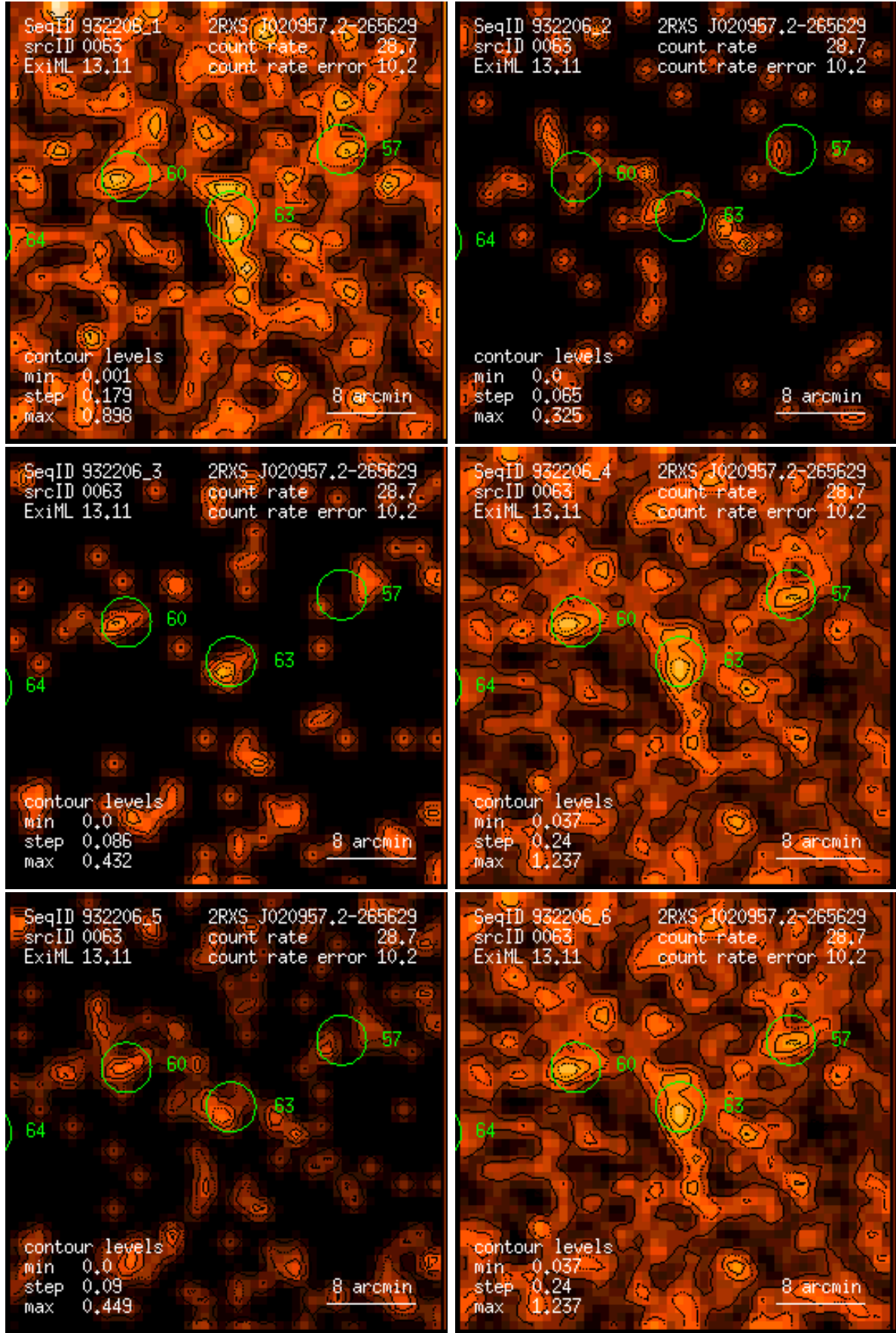
Figure 63: RASS 932206: detection 0063: band rate images, Gaussian filter: (1) PSPC channels 11 – 41, (2) 52 – 90, (3) 91 – 201, (4) 11 – 235, (5) 52 – 201, (6) 11 – 201. Broad band rates in counts/ks. Band rate contour levels in counts/ks/arcmin 2 .
