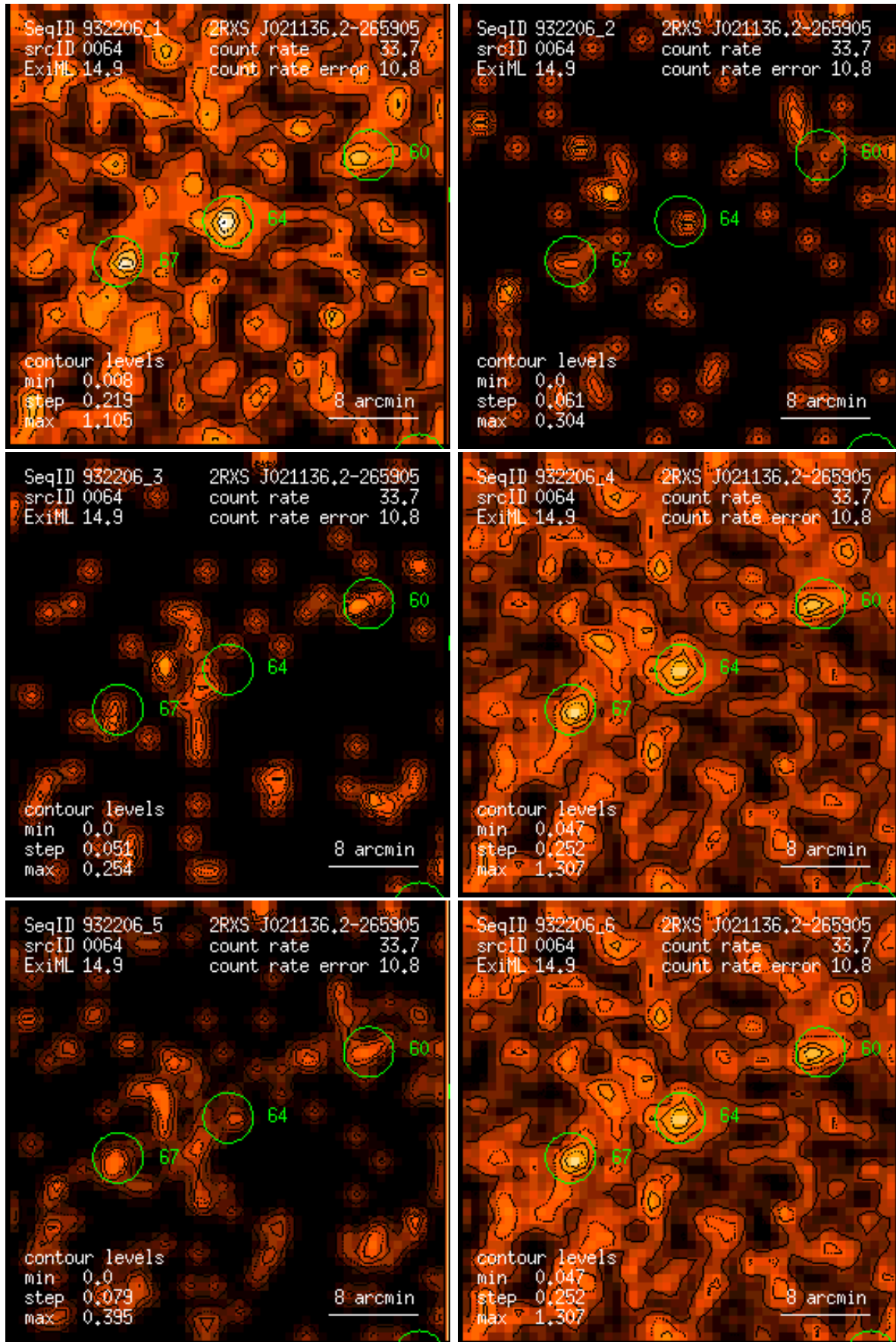
Figure 64: RASS 932206: detection 0064: band rate images, Gaussian filter: (1) PSPC channels 11 – 41, (2) 52 – 90, (3) 91 – 201, (4) 11 – 235, (5) 52 – 201, (6) 11 – 201. Broad band rates in counts/ks. Band rate contour levels in counts/ks/arcmin 2 .
