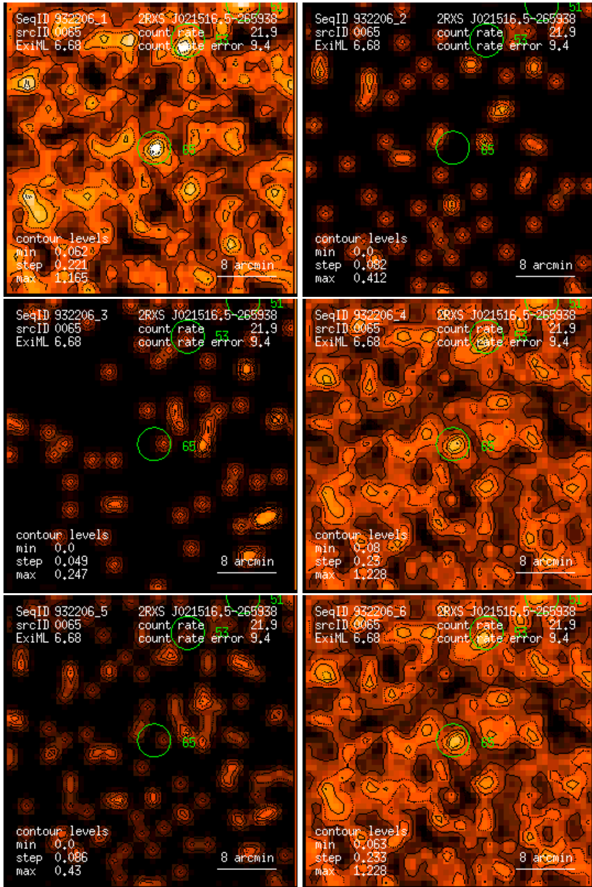
Figure 65: RASS 932206: detection 0065: band rate images, Gaussian filter: (1) PSPC channels 11 – 41, (2) 52 – 90, (3) 91 – 201, (4) 11 – 235, (5) 52 – 201, (6) 11 – 201. Broad band rates in counts/ks. Band rate contour levels in counts/ks/arcmin 2 .
