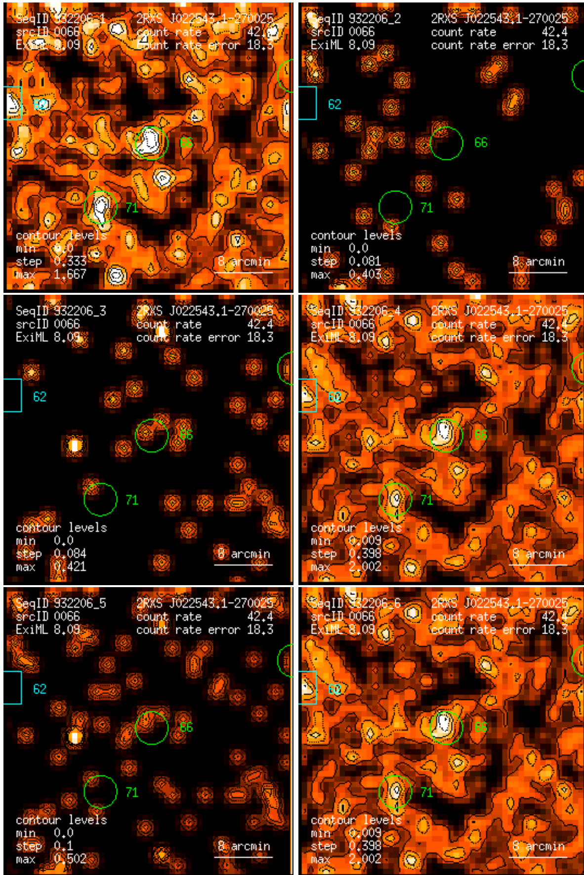
Figure 66: RASS 932206: detection 0066: band rate images, Gaussian filter: (1) PSPC channels 11 – 41, (2) 52 – 90, (3) 91 – 201, (4) 11 – 235, (5) 52 – 201, (6) 11 – 201. Broad band rates in counts/ks. Band rate contour levels in counts/ks/arcmin 2 .
