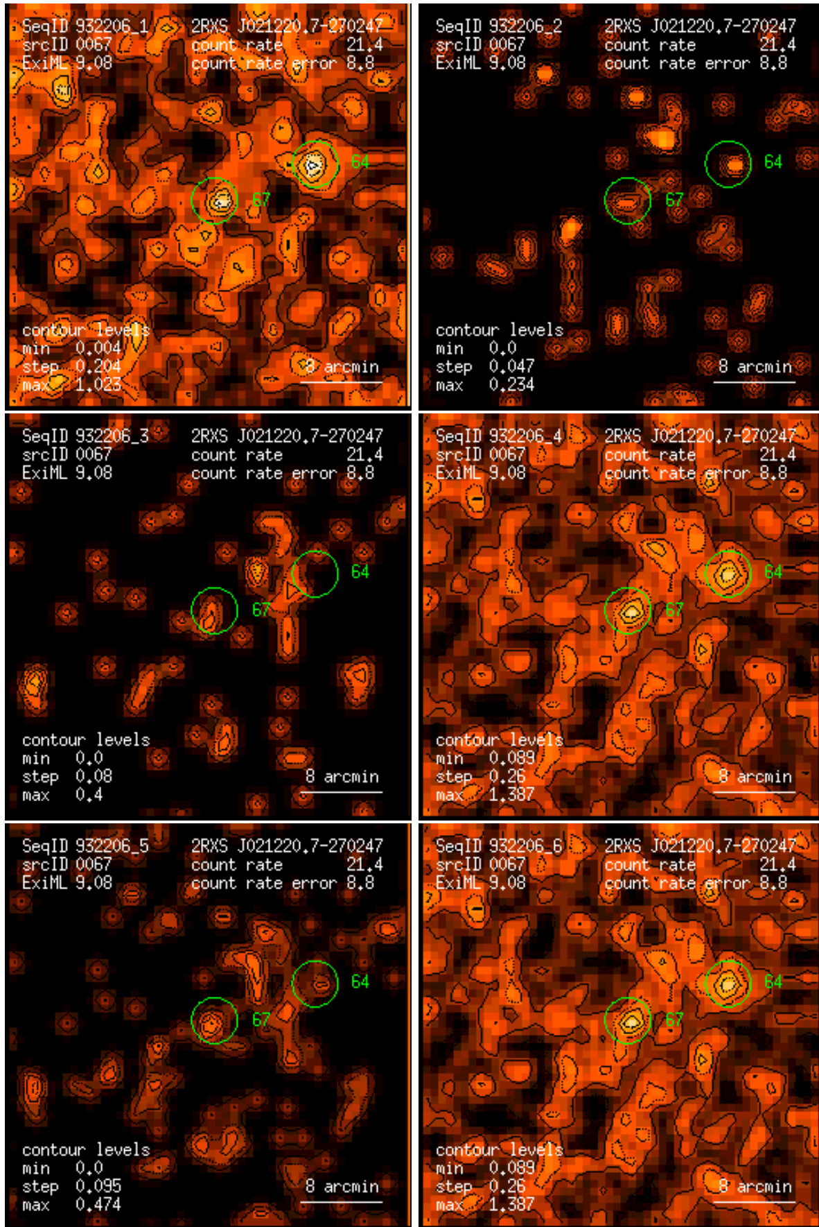
Figure 67: RASS 932206: detection 0067: band rate images, Gaussian filter: (1) PSPC channels 11 – 41, (2) 52 – 90, (3) 91 – 201, (4) 11 – 235, (5) 52 – 201, (6) 11 – 201. Broad band rates in counts/ks. Band rate contour levels in counts/ks/arcmin 2 .
