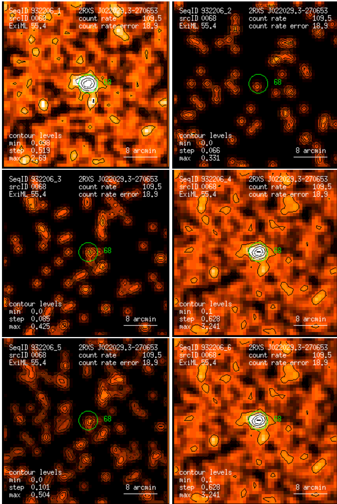
Figure 68: RASS 932206: detection 0068: band rate images, Gaussian filter: (1) PSPC channels 11 – 41, (2) 52 – 90, (3) 91 – 201, (4) 11 – 235, (5) 52 – 201, (6) 11 – 201. Broad band rates in counts/ks. Band rate contour levels in counts/ks/arcmin 2 .
